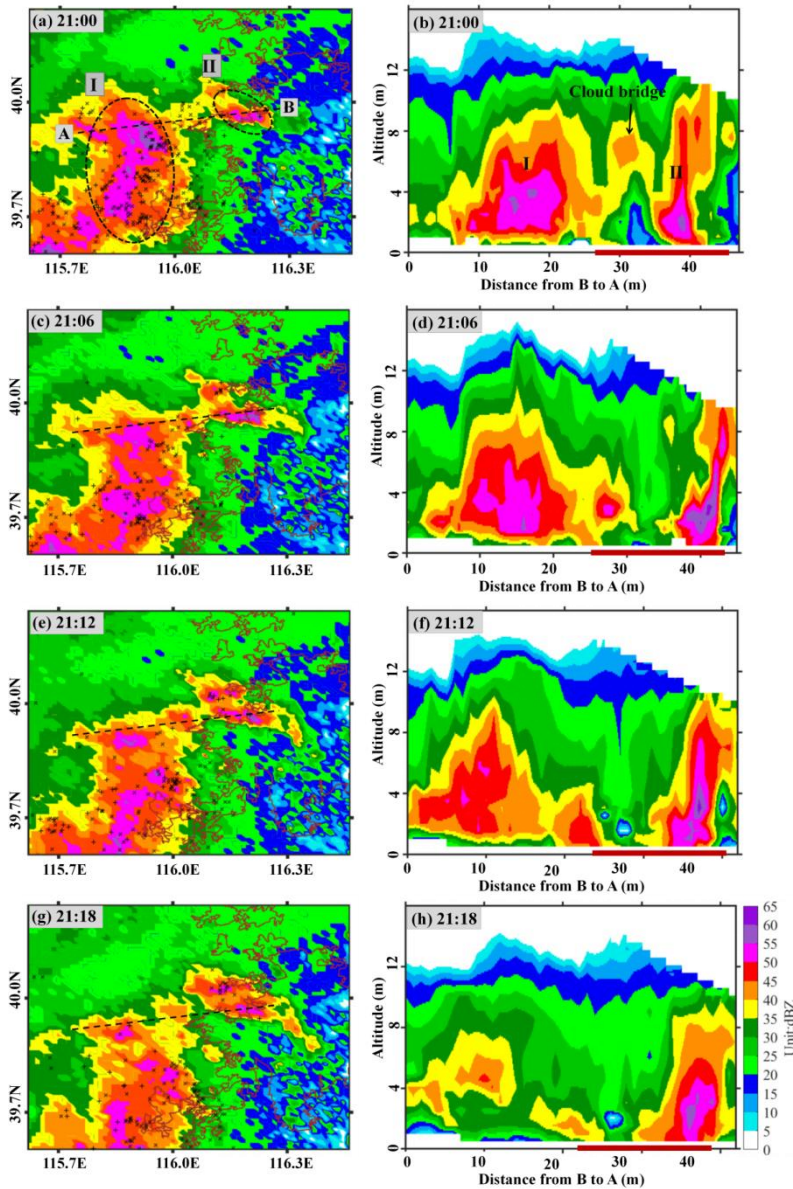
210 Figure 5: The CR product of the "0713" case during the stage of bifurcation, at 21:00 (a-b), 21:06 (c-d), 21:12 (e-f), and 21:18 (g-h) BJT.
