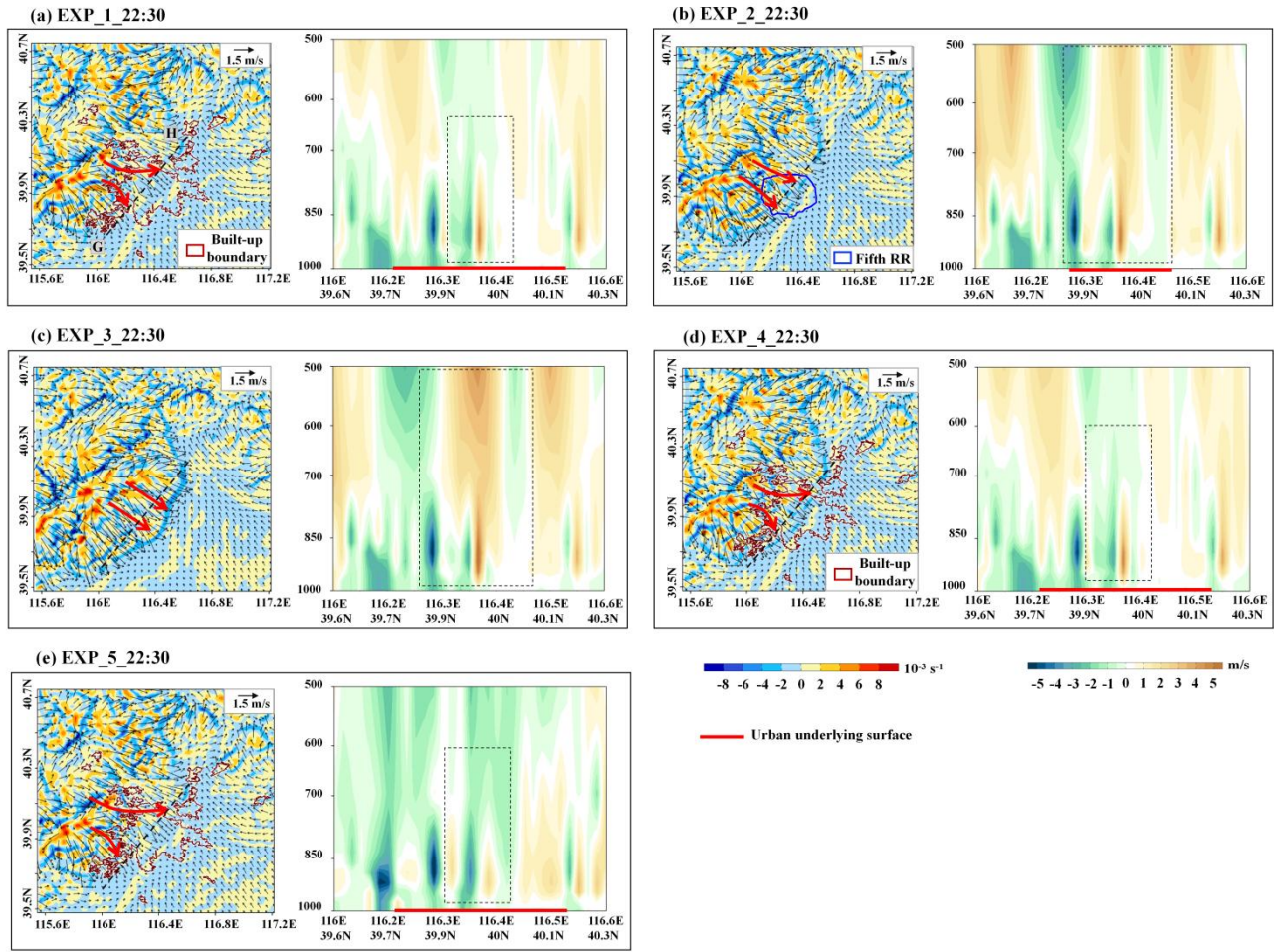
315 Figure 9: Influence of urban underlying surface on near-surface convergence zones simulated by WRF. Figures (a) to (e) represent experiments 1 to 5, respectively. In each set of subfigures, the left subfigure represented the horizontal wind field and divergence field, while the right subfigure depicted the cross-section of vertical velocity along line GH.
