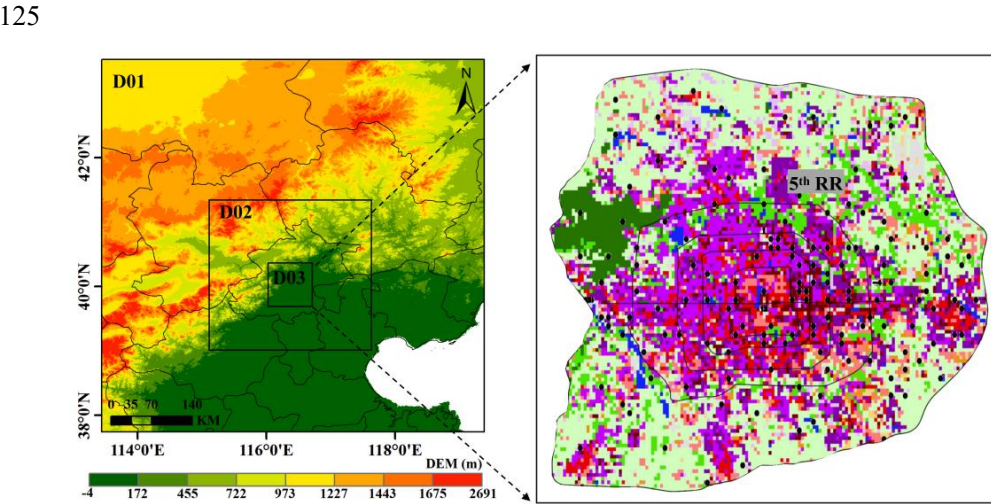
Figure 2: Terrain height distribution and the building types of the WRF mesoscale numerical model.
