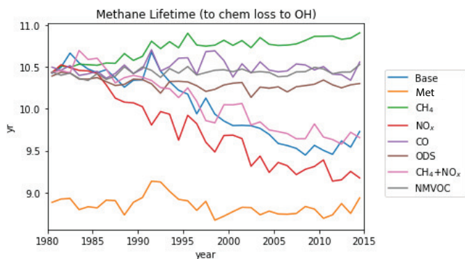
Figure 13. CH 4 lifetime with respect to oxidation by OH for the different model runs. CH 4 lifetime has decreased in the 'Base' run even as CH 4 concentrations have increased, driven by [OH] increases due to increasing NO x emissions.
