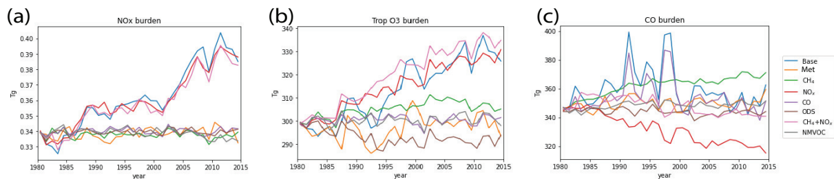
Figure A2. (a) Tropospheric O 3 , (b) NO x and (c) CO burdens for the different model runs.
