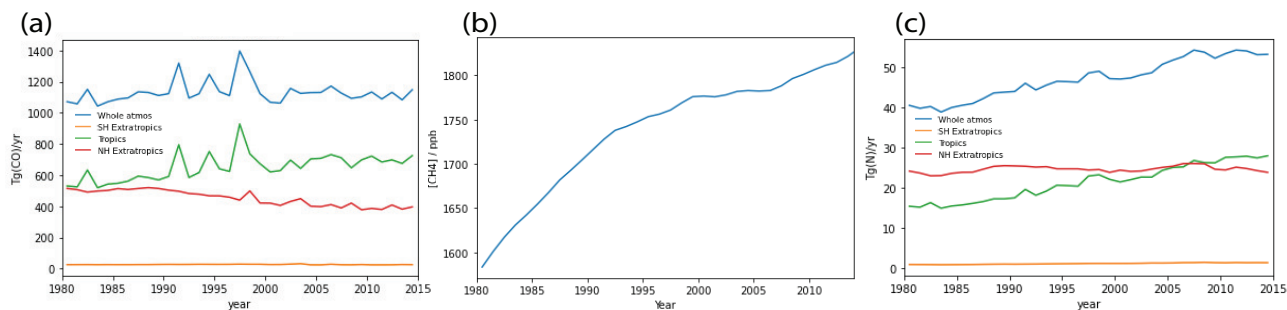
Figure 1. Historical time series of (a) regional CO emissions, (b) CH 4 surface concentrations, and (c) regional NO x emissions used for this study. The Southern Hemisphere (SH) extratropics is defined as 90°S – 30°S, the Tropics as 30°S – 30°N, and the Northern Hemisphere (NH) extratropics as 30°N – 90°N. Globally, CH 4 concentrations have increased by ~ 16%. Non-lightning NO x emissions have also increased by ~ 30% globally over this period, with this increase driven by the Tropics. CO emissions see IAV but little trend globally over this period, but do see a decreasing trend in the NH extratropics offset by an increasing trend in the Tropics.
