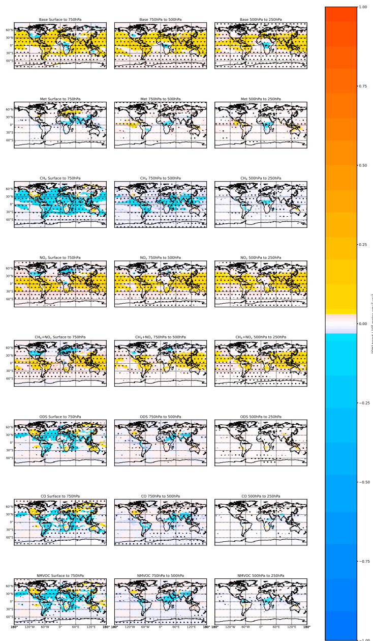
Figure A1. Spatial airmass-weighted tropospheric [OH] trends at different pressure levels for the different runs. Trends and stipples are as per Fig 3.
