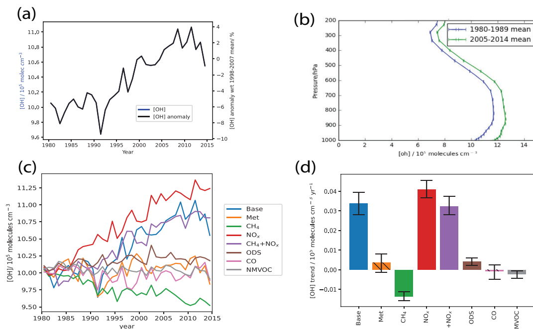
Figure 2. Tropospheric airmass-weighted [OH] (a) time series for the 'Base' run as well as the anomaly with respect to the 1998-2007 mean from 1980 to 2014; (b) 10-year area-weighted mean [OH] at various altitudes for 1980-1989 and 2005-2014 periods; (c) Tropospheric [OH] time series and (d) trends from the Base simulation and from the sensitivity simulations with all ('Met') and individual short-lived emissions held constant at 1980 levels. For (b), error bars represent \pm 1 standard deviation about the mean at each pressure level. For (d), trends are calculated using the Theil-Sen method, and error bars show the 95% confidence interval. Bars are hashed when no significant trend is detected at the 95% level using the Mann-Kendall test. From (a), tropospheric airmass-weighted [OH] has increased by \sim 5\% from 1980 to 2014 in the Base simulation. As seen in (b), the increase in [OH] occurs throughout the depth of the troposphere, but with the largest increase seen from the surface to the lower troposphere, and this could suggest that the increasing [OH] trend is driven by mainly surface drivers. From (c) and (d), we see that globally the [OH] increasing trend is driven by the combined effects of CH 4 and NO x .
