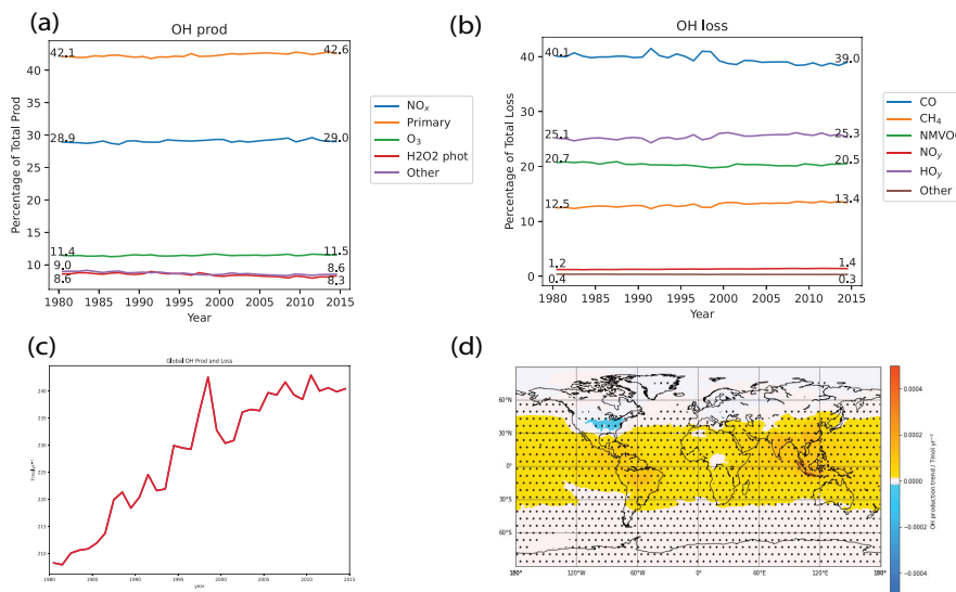
Figure 6. Tropospheric Airmass-weighted OH chemical production and loss terms in the 'Base' run. (a) Evolution of the proportion of each production reaction with respect to the total, and (b) Same but for loss reactions instead. (c) Time evolution of global total production and loss terms (curves overlap because OH is in pseudo steady-state.) (d) Spatial airmass-weighted tropospheric OH chemical production trend over the 1980-2014 period, with stippling and trends as per Fig. 3. From (a) and (b), we see that the relative proportions stay roughly constant throughout the time period, suggesting that all of the reaction terms have increased in tandem with the total, and the values are roughly consistent with Table 1 of Lelieveld et al. (2016). From (c), both global tropospheric airmass-weighted OH production and loss have increased by about 14% by 2014 compared to 1980, showing a clear trend. We also see some IAV throughout the period, with year-on-year changes of up to 2%. Relating these results to the earlier findings, where we saw an increasing [OH] trend, the increasing trend in both production and loss (as they balance each other in steady-state) should therefore be driven by an increasing trend in production, and that in turn should be associated with the net NO x and CH 4 effects. Meanwhile, the IAV observed in the OH concentrations should also be associated with the IAV seen in the production and loss, and this in turn should be affected by meteorological factors, factors that are driven by meteorology like lightning NO x and biogenic VOC emissions, and CO emissions. From (d), we see that spatial chemical production trends matches the spatial [OH] trend plot for the 'Base' run in Fig. 3, suggesting again the role of chemical production (and loss) in driving [OH] trends.
