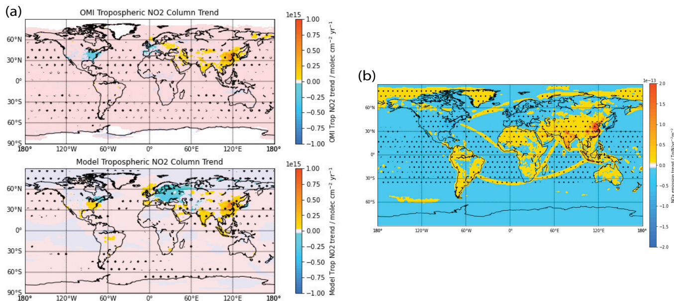
Figure 12. (a) Model comparison of annual mean tropospheric \text{NO}_2 column trends with OMI tropospheric \text{NO}_2 observations over the 2005–2014 period, and (b) \text{NO}_x emission trends over the 2005–2014 period. Trends and stippling are as per Fig. 3. We see that there is general agreement between the emissions and the model tropospheric \text{NO}_2 column. Also, both show significant positive trends over South Asia and Eastern China, and significant negative trends over Eastern USA and Western Europe. These, in turn, are also consistent with the OMI tropospheric \text{NO}_2 column observations. Overall, these findings lend confidence in our model \text{NO}_x trends from 2005 to 2014.
