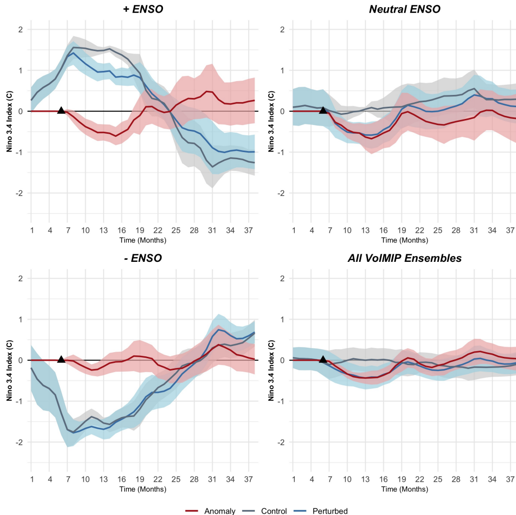
Figure 2. Monthly, seasonally de-trended time series of changes in the monthly Nino 3.4 ENSO index under different ENSO initial conditions and for the full VolMIP ensemble. Positive and negative ensembles show a relaxation of the index response towards mean climatological sea surface temperature conditions. Red shading shows the 95% confidence interval for the anomalous response from control conditions.
