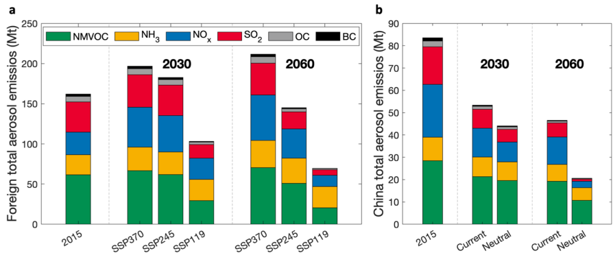
1 2 Figure S1. Future emissions of PM 2.5 -related pollutants in China and in other countries. (a) 3 Emissions for foreign countries within our Flex-Grid simulation domain (11° S–60° N, 30°–150° 4 E) for future years are projected under SSP-RCP scenarios, with updates on base year emissions 5 and the harmonization year in this study. Colors represent the emissions of different pollutants 6 following the legend. (b) Emissions for China for future years are projected with the current- 7 policy scenario and the carbon-neutral scenario. 8
