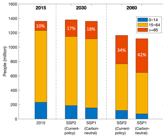
Figure S6. Future population and age structure in China. Total populations in China in 2015 and future years projected under different SSP scenarios (SSP1 corresponds to China’s carbon-neutral scenario; SSP2 corresponds to China’s current-policy scenario). Colors represent different age groups according to the legend. White numbers indicate the fraction of population above the age of 65 in the total population.
