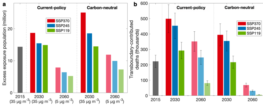
1 2 3 Figure 6. Potential health threats associated with transboundary pollution in China. (a) 4 Population exposed to an annual mean population-weighted PM 2.5 concentration above the goals 5 (35 μg m -3 for 2015 and 2030; 5 μg m -3 for 2060) due to transboundary contributions of PM 2.5 in 6 China under different emission scenarios in China (denoted as text at the top) and in other 7 countries (represented by colors in the legend). (b) Transboundary-contributed 8 premature mortality in China under different emission scenarios in China (denoted as text at the 9 top) and in other countries (represented by colors in the legend). Error bars represent the 95% 10 confidence interval of the RR function. 11
