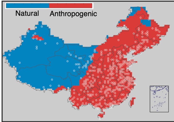
1 2 Figure S3. Anthropogenic emission-dominated grid cells (red) and natural emission-dominated 3 grid cells (blue) at a 0.5^\circ \times 0.625^\circ resolution in China. Circles indicate locations of PM_{2.5} 4 observations used in this study. 5 6 7 8 9 10
