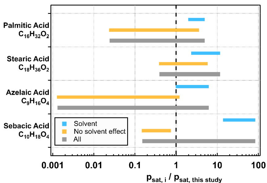
Figure 3. Ranges of normalized p_{\text{sat}} values for palmitic, stearic, azelaic, and sebaccic acids. Each reported p_{\text{sat}} value in literature was normalized to that of our study. The whole range of normalized p_{\text{sat}} of each compound is shown as a grey bar. The group of samples potentially impacted by solvents is shown as a blue bar, while that with no impact from solvents is shown as a yellow bar. Note that data from Bilde et al. (2015) shown in Fig. 2 were not included for these analyses.
