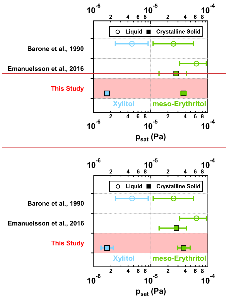
370 Figure 4. Measured p_{\text{sat}} values from this study (rectangle in red shaded area) together with those reported in literature for meso-erythritol (green) and xylitol (blue). For the p_{\text{sat}} values from this study, they were estimated using \alpha = 1 , with error bars including \pm 50\% variation in the chosen \sigma and the fitting uncertainties (i.e., 95 % CrIs).
