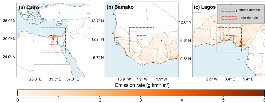
Figure 2. Domain setup of the WRF simulations over Cairo (Egypt), Bamako (Mali) and Lagos (Nigeria). The inner domain (red) spans 315x315 km 2 around the city at 3 km resolution. The middle (black) and outer (full figure) domain cover 893x893 km 2 and 2673x2673 km 2 at 9 and 27 km resolution respectively. All panels show the emission rates from the DACCIWA inventory.
