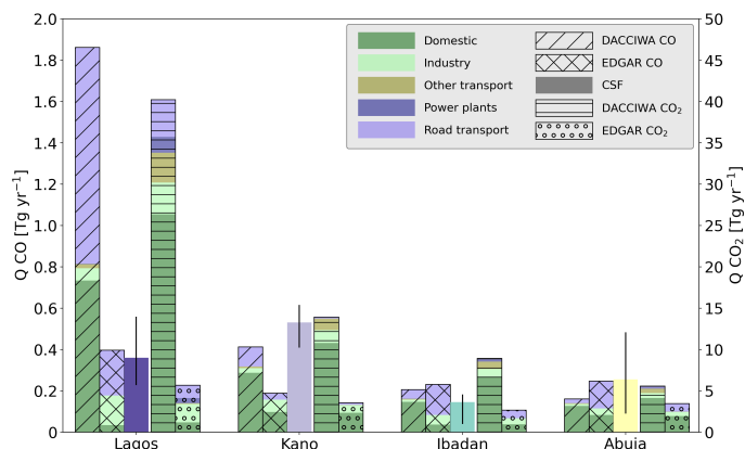
Figure 9. Comparison between the TROPOMI CO emission estimates and EDGAR and DACCIIWA CO and \text{CO}_2 for four cities in Nigeria with the same color scheme as Fig. 7. The differences between the two inventories in \text{CO}_2 emission rates indicate a different spatial allocation - based on gridded activity data- of the national totals.
