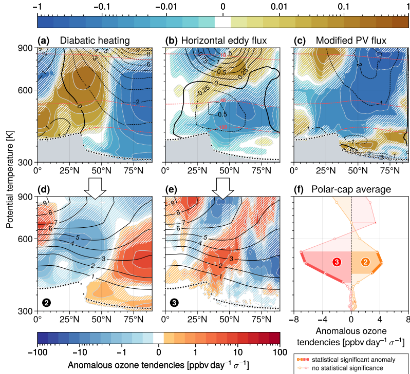
Figure 7. (a) Anomalous diabatic heating rates \overline{Q^*} (in \text{K day}^{-1} ) and (b) horizontal eddy ozone transport \overline{\hat{v}\rho_\theta\hat{\chi}}/\overline{\rho_\theta} (in \text{ppmv m s}^{-1} ) regressed on the T100 index (ERA-Interim). (c) The corresponding regression map for the modified PV flux \overline{\hat{v}\rho_\theta\hat{\Pi}}/\overline{\rho_\theta} (in \text{PVU m s}^{-1} ) is added for comparison. Details as in Fig. 3. (d, e) T100 regression maps for the anomalous tendencies ② and ③ from eq. (4). Here, the black contours show the ozone DJF climatology (in \text{ppmv} ). Note uneven color contour intervals with linear spacing for values within \pm 0.01 (top row) and \pm 1 \text{ ppbv day}^{-1} \sigma^{-1} (bottom row), respectively, and logarithmic spacing outside those ranges. The anomalous ozone tendencies seem to be weak in the lowermost stratosphere and increase strongly for altitudes higher than 400 K due to increased wave forcing above that isentrope as indicated by the anomalous equatorward PV fluxes in (c). Weak positive ozone tendencies due to enhanced diabatic cooling directly above the tropopause in (d) probably arise from an increase in static stability there, e. g., as observed for sudden stratospheric warmings (Grise et al., 2010; Son et al., 2011; Wargan and Coy, 2016), or can be explained as a second-order feedback reacting to changes in the vertical ozone gradients. (f) Polar-cap averaged tendencies, \langle \partial_t \bar{\chi}^* \rangle_\phi for \phi \geq 60^\circ\text{N} , regressed on the ERA-Interim T100 index. Thick solid lines mark isentropes with statistically significant anomalies. All results are for ERA-Interim, DJF 1980–2016.
