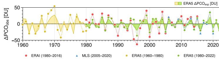
Figure 9. (a–c) Maps of interannual ozone variability, based on local sample standard deviations relative to the ozone DJF climatology, for ERAI, MLS and ERA5. The thick dotted lines show the mean thermal tropopause derived from ERAI data. For ERAI and ERA5, extreme ozone variations (indicated by red shading and stippling) are caused by statistical outliers. (d) Observed polar-cap averaged partial column ozone anomalies \Delta\text{PCO}_{\text{obs}} per DJF winter season (line plots) for the different datasets ERAI, MLS and ERA5 data and, for comparison, explained partial column ozone \Delta\text{PCO}_{\text{exp}} for ERA5 (area plots). See the text for details on the computation.
