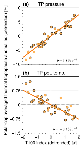
Figure 6. (a) Polar-cap averaged thermal tropopause (TP) pressure regressed on the T100 index (ERA-Interim, DJF 1980–2016), with slope b = 3.8 \% \sigma^{-1} from a linear least-squares fit and correlation r = 0.95 . Much less co-variability is found in (b) for polar-cap TP potential temperature ( r = -0.80 ).
