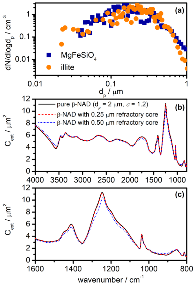
1455 Figure 11: Influence of refractory inclusions on the infrared extinction spectrum of \beta -NAD particles. (a) Measurements of the size distribution of pure \text{MgFeSiO}_4 and illite particles dispersed with a rotating brush generator and introduced into the AIDA chamber. The size spectra were merged from the recordings of a scanning mobility particle sizer (SMPS, TSI) and an aerodynamic particle spectrometer (APS, TSI). In order to convert measured mobility and aerodynamic diameters into the equal-volume sphere diameter, d_p , we used values of 2.6 \text{ g cm}^{-3} for the particle density and 1.4 for the dynamic shape factor. (b) Infrared extinction cross sections of pure, log-normally distributed spherical \beta -NAD crystals with a count median diameter of 2 \mu\text{m} and a mode width of 1.2 (black) in comparison with core-shell Mie simulations in which the centre of the \beta -NAD particles was replaced by spherical refractory inclusions with diameters of 0.25 (red dashed ) and 0.50 \mu\text{m} (blue dotted ). Note that the black line is almost identical to the red dashed line and therefore difficult to see. (c) Expanded view of the extinction cross sections from panel (b) between 1600 and 800 \text{cm}^{-1} .
