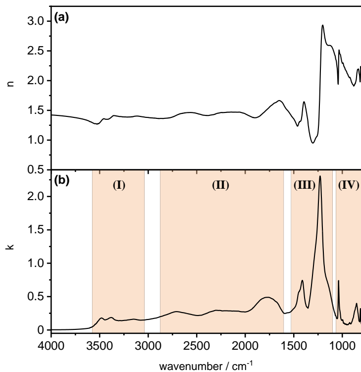
1425 Figure 8: Newly derived data set of mid-infrared optical constants for \beta -NAD. (a) Real part of the complex refractive index ( n spectrum). (b) Imaginary part of the complex refractive index ( k spectrum). The four spectral regions highlighted in part (b) are discussed in the text.
