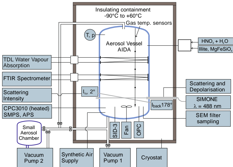
1365 Figure 1: Schematic diagram of the instrumentation of the AIDA aerosol and cloud chamber facility. The instruments (and their respective abbreviations) used in this work are described in more detail in Sects. 2.1 and 2.2.
