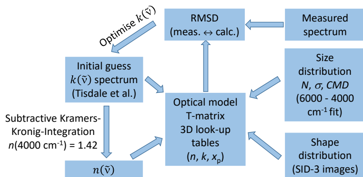
1380 Figure 3: Retrieval scheme for deriving the optical constants of \beta -NAD. See Sect. 2.3 for more details and explanation of abbreviations.
