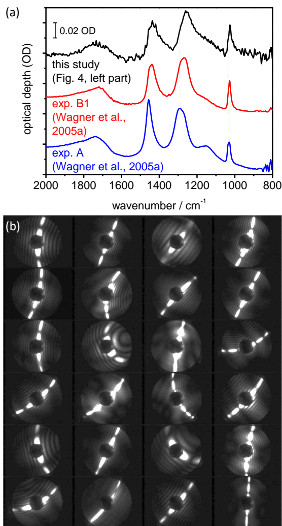
1410 Figure 6: (a) Shape-dependent infrared spectral signature of airborne \alpha -NAD crystals. The blue-coloured spectrum was recorded 1415 during exp. A from Wagner et al. (2005a) where the \alpha -NAD particles were generated by shock-freezing a gaseous nitric acid – water mixture. In exp. B1 from Wagner et al. (2005a), the \alpha -NAD crystals were formed by homogeneous nucleation from slowly evaporating supercooled \text{HNO}_3/\text{H}_2\text{O} solution droplets at 193 K. A similar long-term crystallisation experiment was performed in this study at 190 K (see Fig. 4, left part), and the infrared spectrum of the nucleated \alpha -NAD crystals is shown in black. Vertical green dotted lines indicate the shifts in band positions between the different spectra. Individual spectra have been offset for clarity. (b) SID-3 measurements: Representative two-dimensional scattering patterns of the \alpha -NAD crystals that formed during the long-term crystallisation experiment at 190 K from this study.
