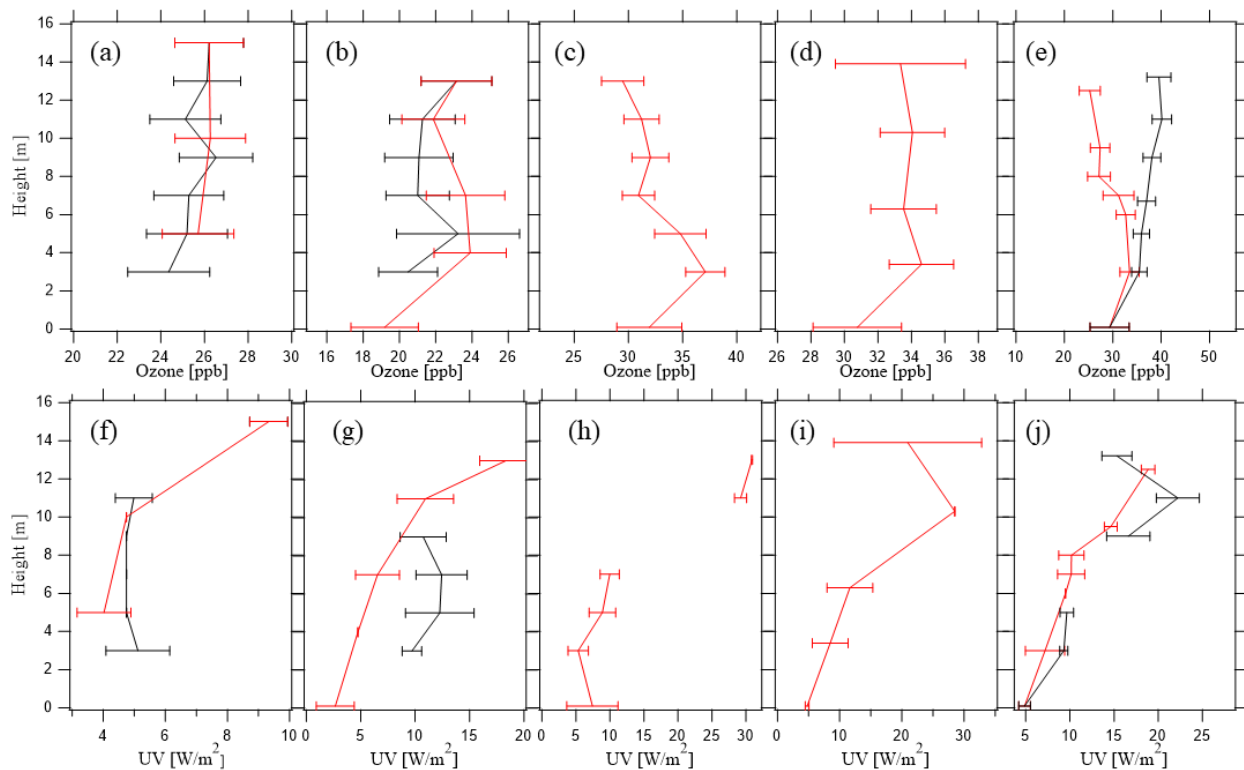
600 Figure 5: Vertical profiles of ozone (a-e) and UV (f-j) from the tower pulley system within the canopy ( h_c = 19 m). Dates (all 2017) and approximate times are: 18:00, 22 Jul (a,f); 17:00, 24 Jul (b,g); 15:00, 25 Jul (c,h); 15:00 to 18:00, 26 Jul (d,i); 12:00, 27 Jul (e,j). Black lines show ascending measurements, and red lines show descending measurements. Error bars show standard deviations at each height within each 15-min measurement period.
