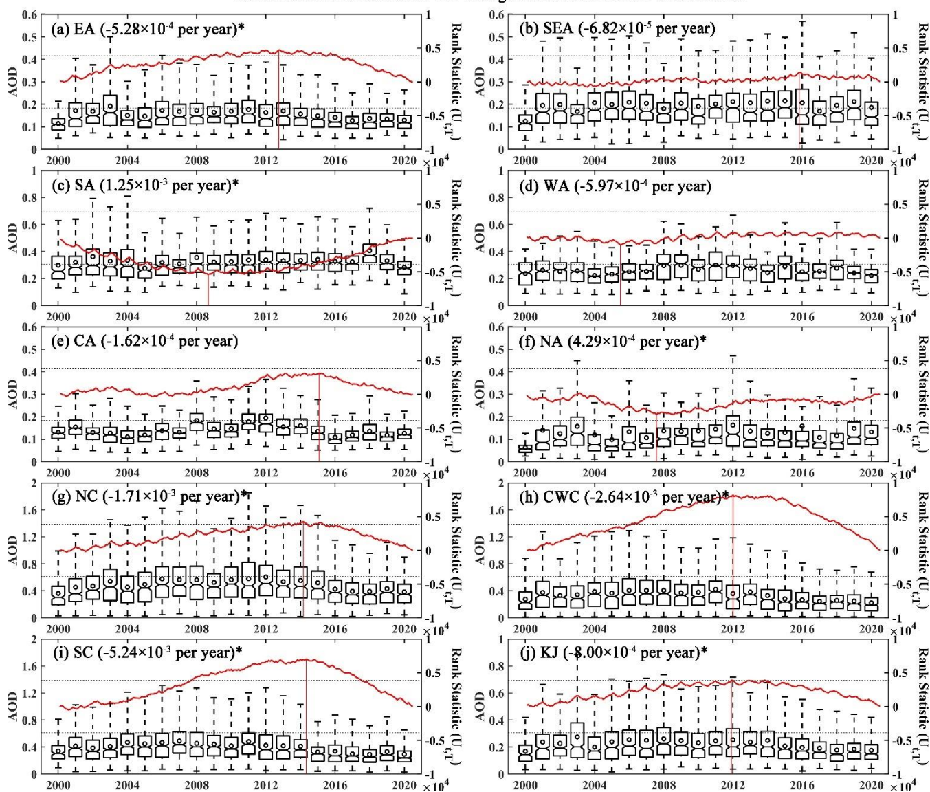
Distributions of Annual AOD and Change Points from MODIS Observations
