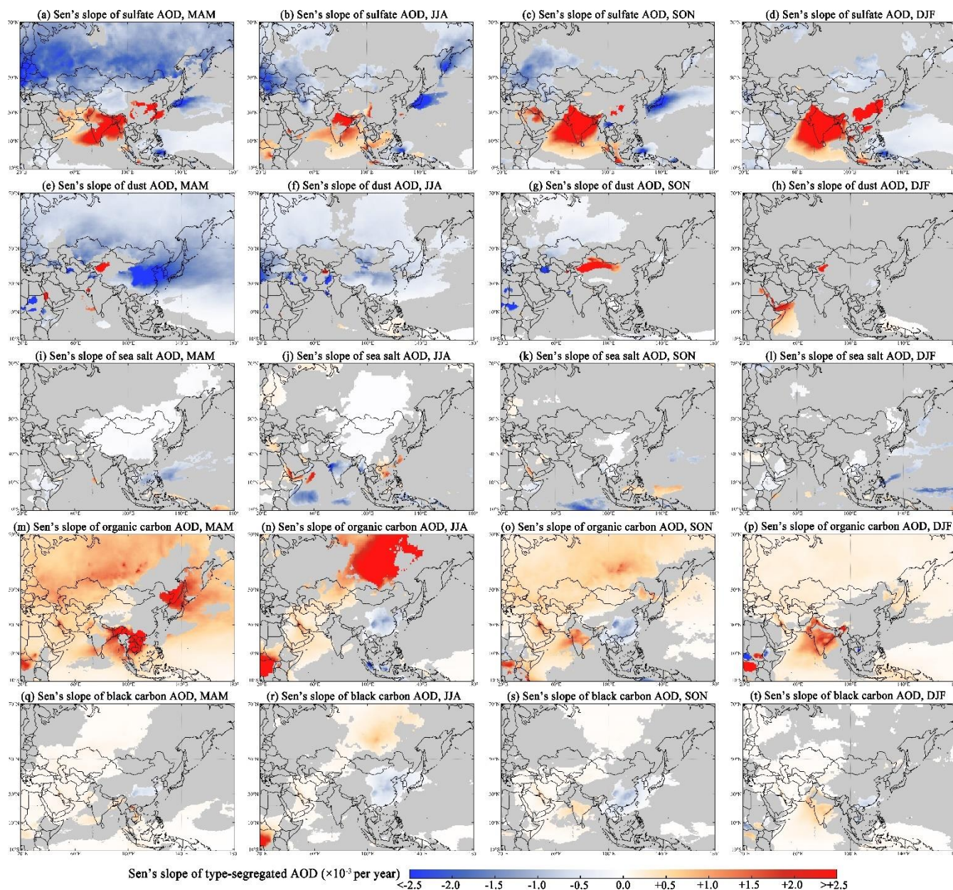
Figure 9. Long-term trends of seasonal sulphate, dust, SS, OC, and BC AOD in Asia from 2000 to 2020. These type-segregated AODs are obtained from MERRA-2 reanalysis data. All the points have passed the significance test ( p < 0.05 ). Gray colour represents that the trend is not significant.
