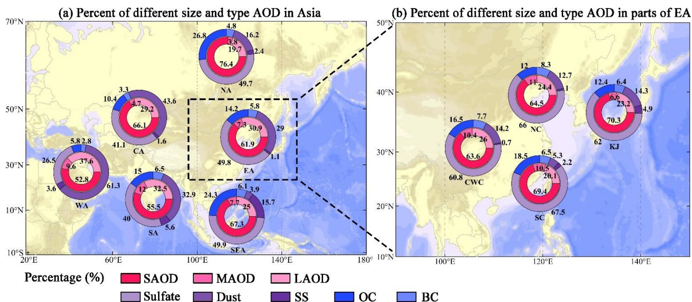
Figure 6. Percentage of size-segregated AOD (SAOD, MAOD, and LAOD) and type-segregated AOD (sulphate, dust, SS, OC, and BC AOD) in the total AOD over (a) Asia and (b) parts of EA.
