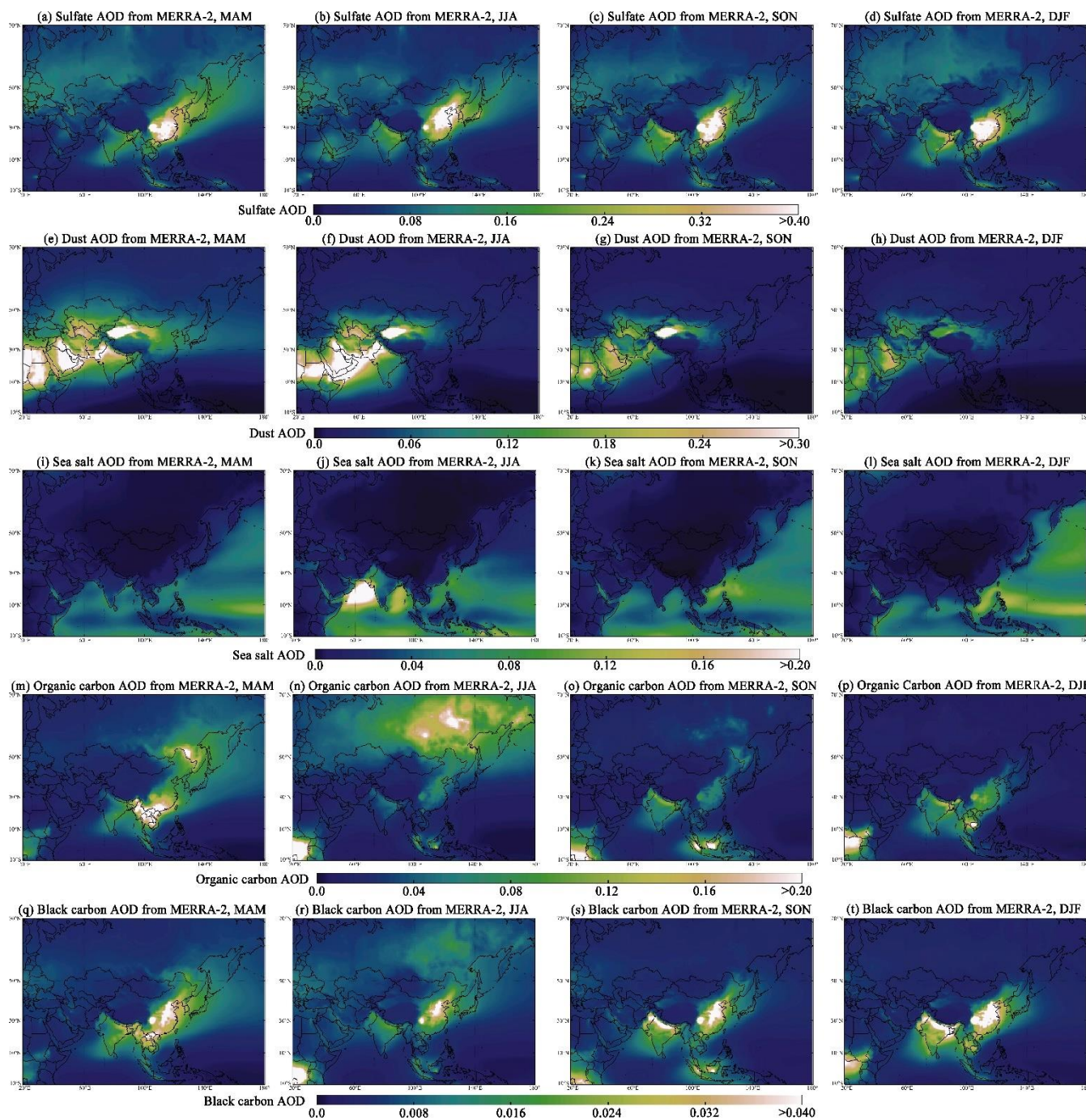
425 Figure 5. Spatial distributions of seasonally sulphate, dust, SS, OC, and BC AOD obtained from MERRA-2 reanalysis data in Asia from 2000 to 2020.
