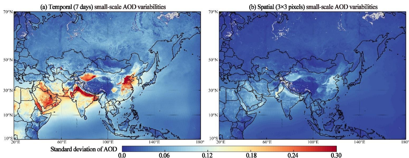
Figure 11. Temporal and spatial small-scale variabilities of AOD. The temporal standard deviation of AOD was calculated 600 in a range of 7 days, while the spatial standard deviation of AOD was calculated by a 3×3 pixel sliding window.
