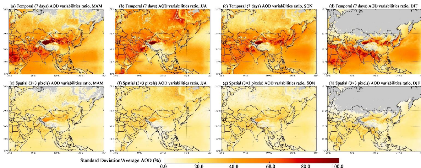
Figure 12. Temporal and spatial small-scale relative variabilities of AOD (standard deviation/average AOD). The temporal standard deviation of AOD was calculated in a range of 7 days, while the spatial standard deviation of AOD was calculated by a 3×3 pixel sliding window.
