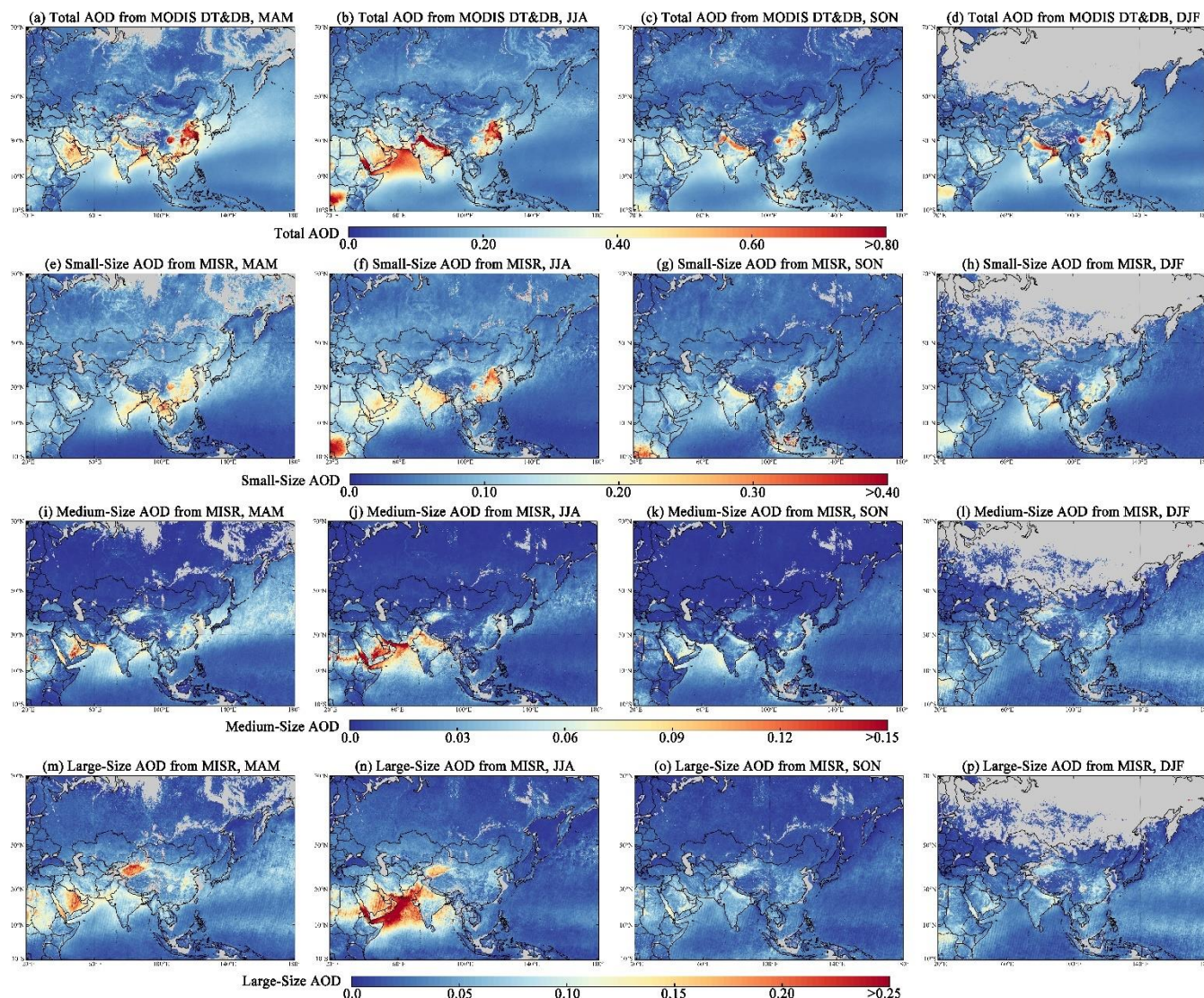
Figure 4. Spatial distributions of seasonal AOD, SAOD, MAOD, and LAOD obtained from MODIS and MISR aerosol products in Asia from 2000 to 2020. The AOD was from MODIS C6.1 DT&DB dataset and the size-segregated AOD was from MISR V23 aerosol products.
