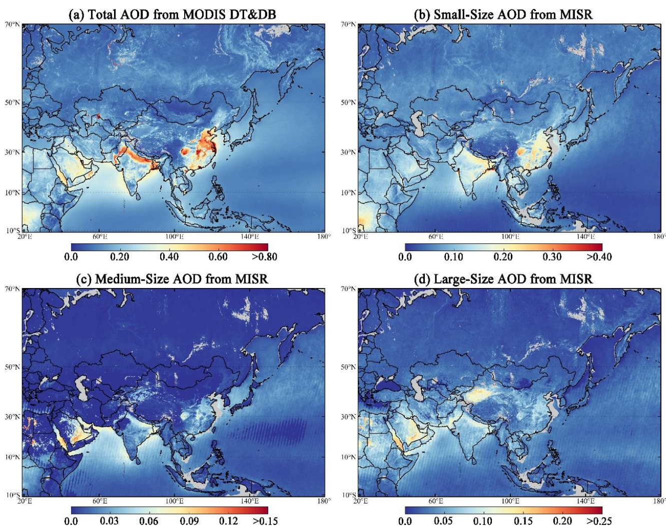
380 Figure 3. Spatial distributions of annual average of (a) AOD, (b) SAOD, (c) MAOD, and (d) LAOD in Asia from 2000 to 2020. The total AOD was from MODIS C6.1 DT&DB dataset and the size-segregated AOD was from MISR V23 aerosol products.
