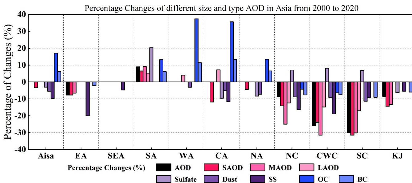
560 Figure 10. Total percent changes in different size and type AOD from 2000 to 2020. Only trends that pass the significance test ( p < 0.05 ) are displayed in this figure.
