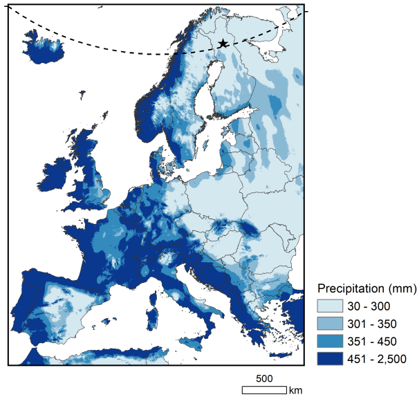
Figure 1. Overview of the geographical location of the experiment setup in Sodankylä, Finland (black star), which is just above the Arctic Circle (dashed line). The average seven-month total precipitation (in mm) for the colder months per year (January-April and October-December) in the period 1970–2000 are shown in the map derived from the monthly climate data from WorldClim (Fick and Hijmans, 2017, see also https://www.worldclim.org/data/worldclim21.html , last access: 31 January 2022).
