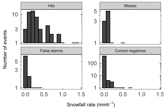
Figure A7. Snowfall rate by intervals measured optically during the events grouped by hits , misses , false alarms , and correct negatives based on the criterion running mean RH_{\text{ice}} \geq 97\% throughout the lower 2.7 km to predict snowfall. The y-axis scale for each panel is different.
