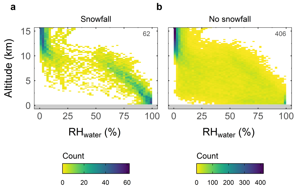
Figure A5. Same plot as Fig. 5, but for RH water .
