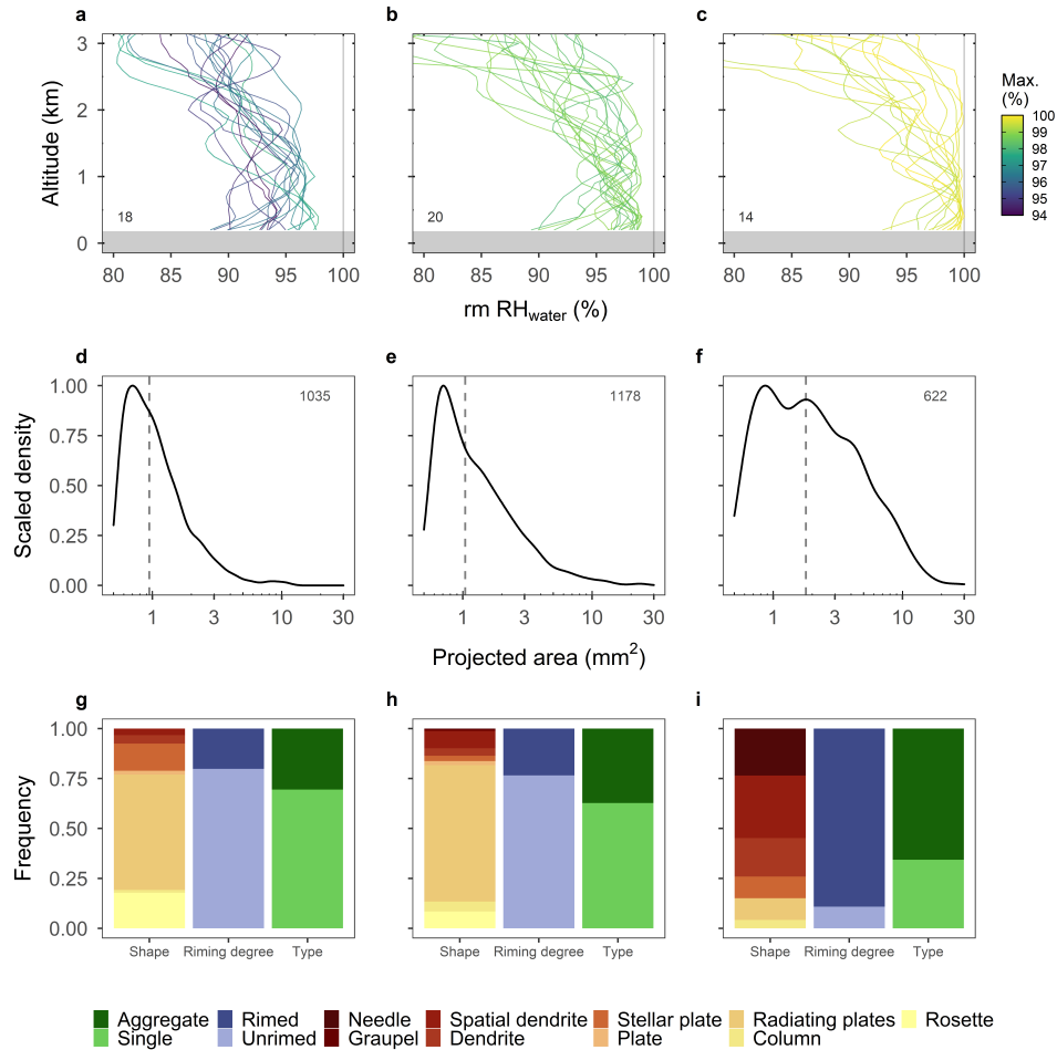
Figure 9. (a, b, c) Running mean RH_{\text{water}} profiles coinciding with snowfall and running mean RH_{\text{ice}} \geq 97\% throughout the lower 2.7 km (52 events) grouped by the maximum running mean RH_{\text{water}} . The maximum running mean RH_{\text{water}} along the altitude profile is shown in colour. (a) Profiles with a maximum running mean RH_{\text{water}} < 98\% . (b) Profiles with a maximum running mean RH_{\text{water}} \geq 98\% and < 99\% . (c) Profiles with a maximum running mean RH_{\text{water}} \geq 99\% . For each panel, the number of profiles is indicated in the left bottom corner. (d, e, f) The scaled density of ice particles by projected area ( \text{mm}^2 ). All the analysed ice particles of the profiles in the above lying panel were considered. The dashed vertical line indicates the median area. The number of analysed ice particles is indicated by the number provided in the upper right corner. During the 52 snowfall events, a total of 2835 ice particles were analysed. (g, h, i) Same as Fig. 8, but considering only the specifiable ice particles coinciding with the events of the above lying panels.
