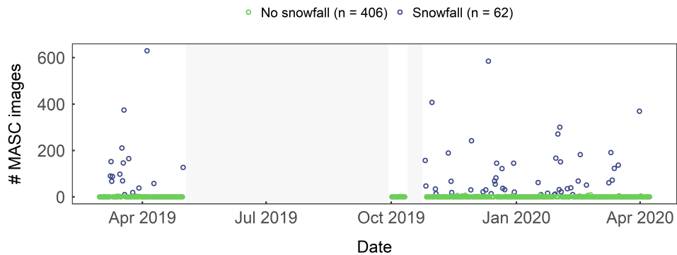
Figure A3. The number of images with objects larger than 0.54 \text{ mm}^2 captured by the operational MASC instrument during coinciding radiosonde profiles from 28 February 2019 to 7 April 2020. Radiosondes were launched twice a day, at 11:30 and 23:30 UTC. Images considered were captured within a time span of 15 minutes before each radiosonde launch. Cases (i.e. 15-min time intervals) with 10 or more of such images are classified as snowfall events ( n = 62 , blue dots). The others are classified as no-snowfall events ( n = 406 , green dots). No data (gray area) was collected in the summer months (May to September) and during a technical interruption between 11 and 25 October 2019.
