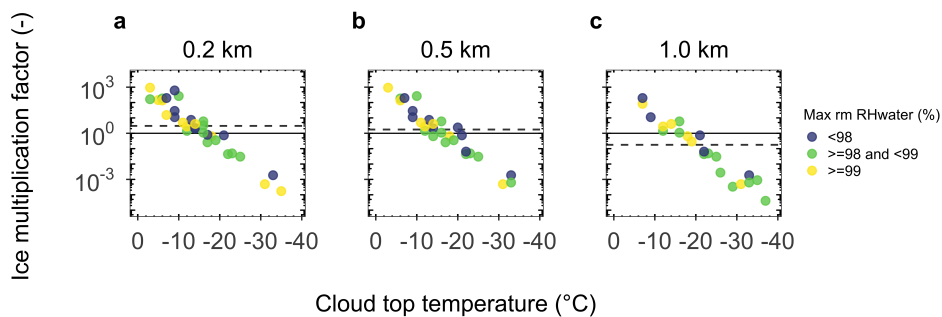
Figure 12. The ice multiplication factor versus cloud top temperature ( ^{\circ}\text{C} ) for each of the 52 snowfall events (coinciding with running mean RH_{ice} \geq 97\% throughout the lower 2.7 km) that were associated with cloud top temperatures warmer than -38 ^{\circ}\text{C} determining the highest possible seeder-feeder cloud using a distance threshold of (a) 0.2 km, (b) 0.5 km, and (c) 1.0 km. The colors are indicative of the associated maximum running mean RH_{water} ( < 98\% , blue; \geq 98\% and < 99\% , green; \geq 99\% , yellow). The median ice multiplication factor is shown by the dashed line. The solid line is drawn at an ice multiplication factor of 1.
