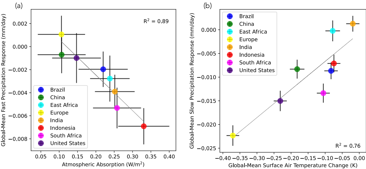
Figure 2. The total global-mean precipitation response to emissions from each region can be decomposed in the (a) global-mean fast precipitation response (mm/day, y-axis), which is strongly correlated with the global-mean change in atmospheric absorption (W/m², x-axis), and the (b) global-mean slow precipitation response (mm/day, y-axis), which is strongly correlated with the global-mean change in surface temperature (K, x-axis). Error bars provide the 95% confidence interval ( \pm 1.96\sigma ).
