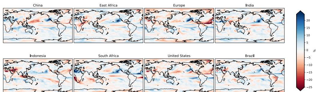
Figure A2. Annual-mean precipitation responses to identical total aerosol emissions within each of the 8 perturbation regions is given in terms of percent change relative to the climatological precipitation in each grid cell taken from the control simulation.
