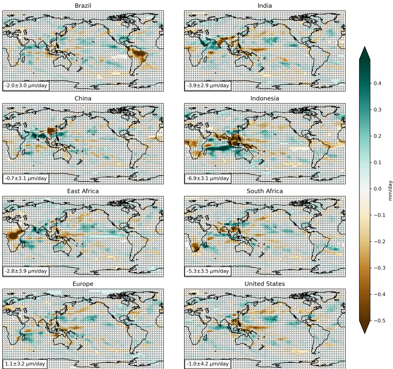
270 Figure 5. Spatial distribution of the change in fast precipitation rate (mm/day) due to the addition of an identical amount and composition of aerosol emissions in each of the 8 regions. Gridlines indicates regions where the changes are not statistically significant at the 95% confidence level via a two-sided t test. Global mean fast precipitation rate change and 95% confidence intervals ( \pm 1.96\sigma ) in \mu\text{m/day} are shown in the bottom left corner of each map.
