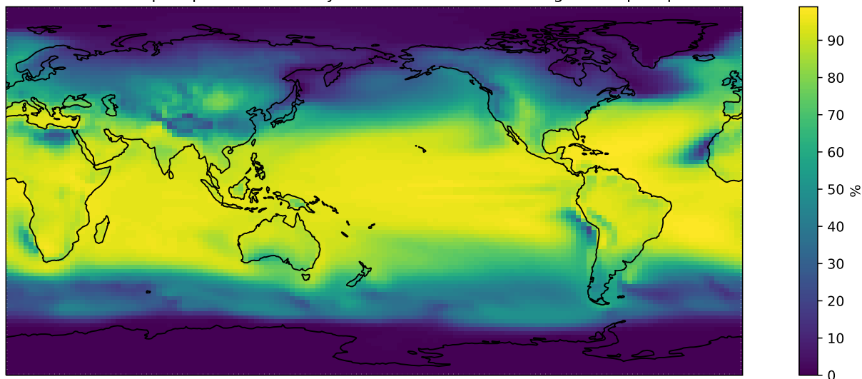
Figure A3. The percent of total precipitation in each grid cell in the control simulation that is derived from convective precipitation as opposed to large-scale precipitation is shown.
