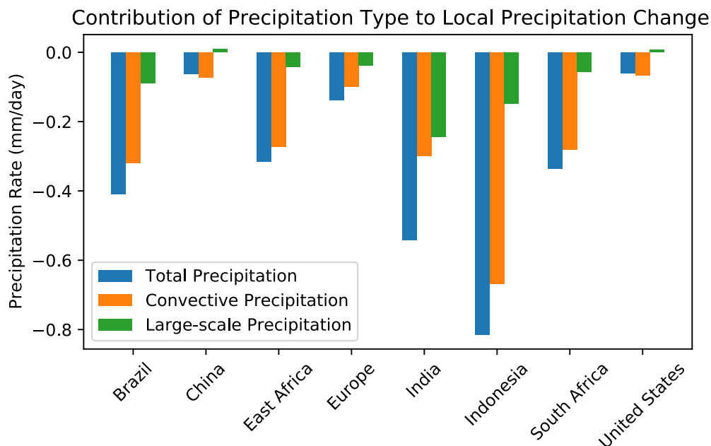
Figure A4. The relative contribution of convective precipitation change (mm/day, orange) and large-scale precipitation change (mm/day, green) to the total local precipitation response (mm/day, blue) within each of the 8 perturbation regions in response to emissions within that region are shown.
