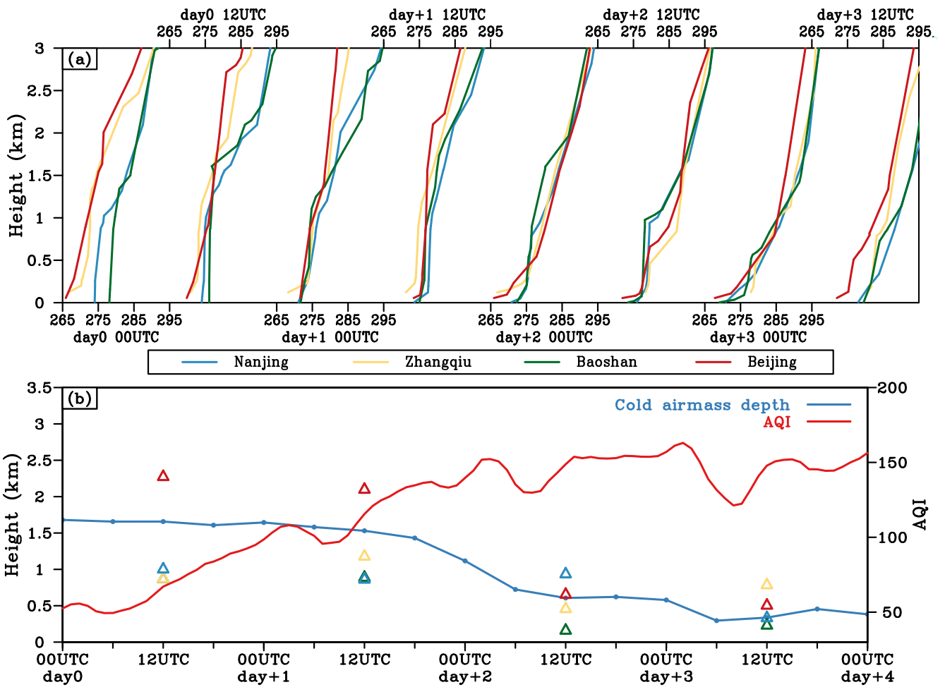
Figure 7: (a) Vertical profiles of potential temperature at four stations (from north to south: Beijing, Zhangqiu, Nanjing, Baoshan) during a CAO rapid event from 14 to 17 Dec 2016. (b) Time series of the regional averaged cold air mass depth and the AQI in NEC and MLH (colored triangles) at four stations during a CAO_rapid event from 14 to 17 Dec 2016.
