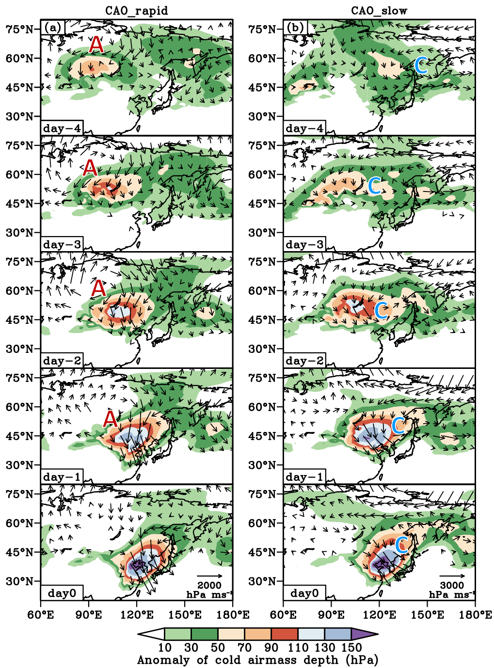
605 Figure 14: Large-scale anomalies of cold airmass depth (shading) and cold airmass flux (vectors) in the initial stage from day -4 to 0. (a) and (b) are composited by the CAO_rapid events and CAO_slow events, respectively.
