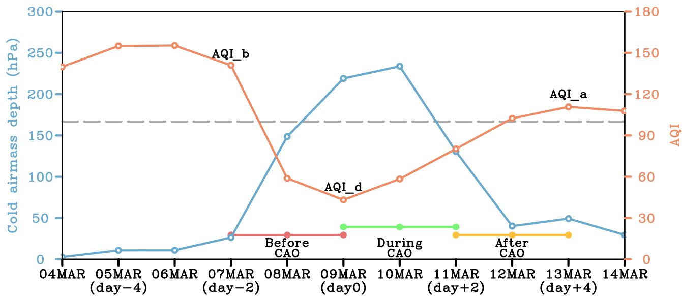
Figure 1: Time series of the regional averaged cold airmass depth (blue line) and AQI (orange line) in NEC (114°–122°E, 30°–40°N). The gray dashed line denotes the threshold value of the cold airmass depth.
