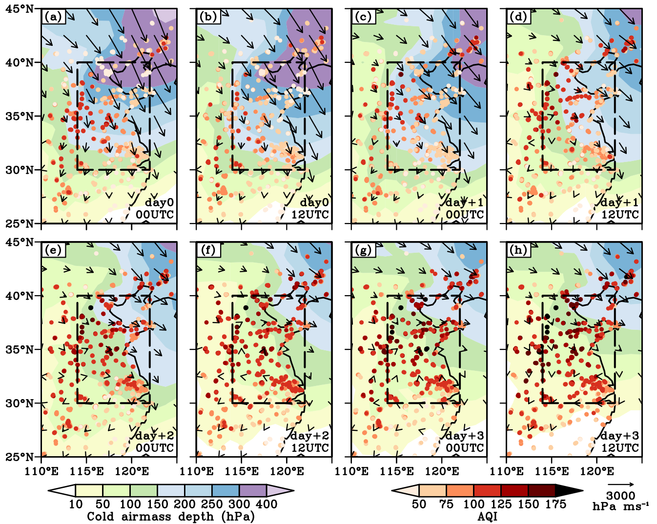
Figure 5: Spatial distributions of the composited cold air mass depth (shaded), horizontal fluxes of the cold air mass (black vectors), and AQI (colored dots) during CAO_rapid events. The black boxes denote the NEC (114°–122°E, 30°–40°N).
