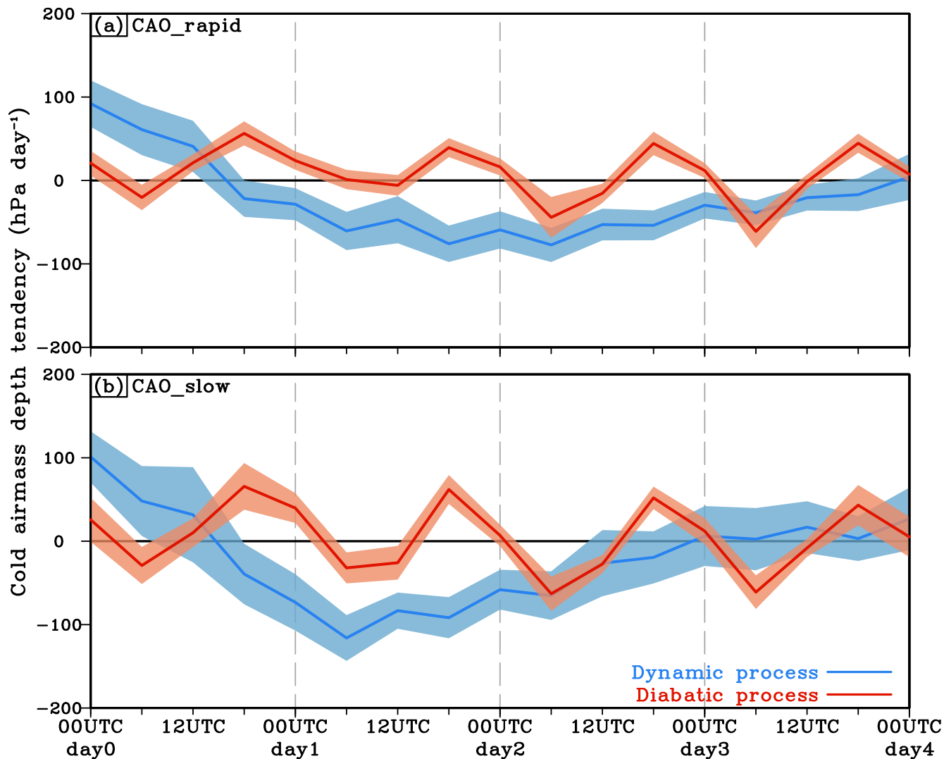
600 Figure 13: Evolutions of the spatially averaged (NEC: 114°–122°E, 30°–40°N) cold air mass depth tendency during CAOs. Blue and red lines denote the contributions of dynamic and diabatic processes to the tendency of cold air mass depth, respectively. (a) and (b) are composited by the CAO_rapid events and CAO_slow events, respectively. Shading represents the 95% confidence interval of the composited mean value.
