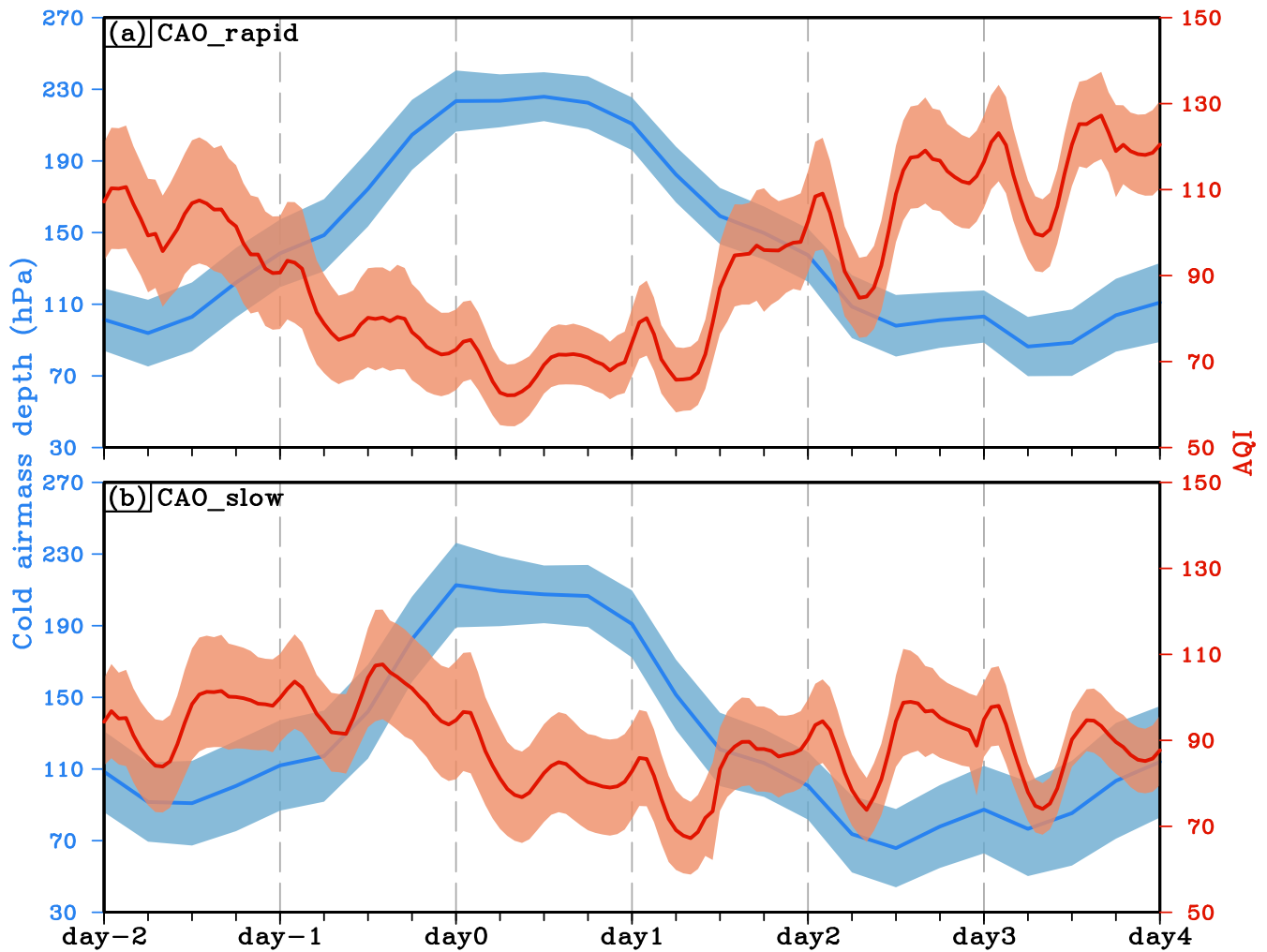
Figure 4: Evolutions of spatially averaged (NEC: 114°–122°E, 30°–40°N) cold air mass depth and AQI during CAOs. (a) and (b) are composited by the CAO_rapid events and CAO_slow events, respectively. Blue lines and red lines denote the cold air mass depth and AQI, respectively. Shading represents the 95% confidence interval of the composited mean value.
