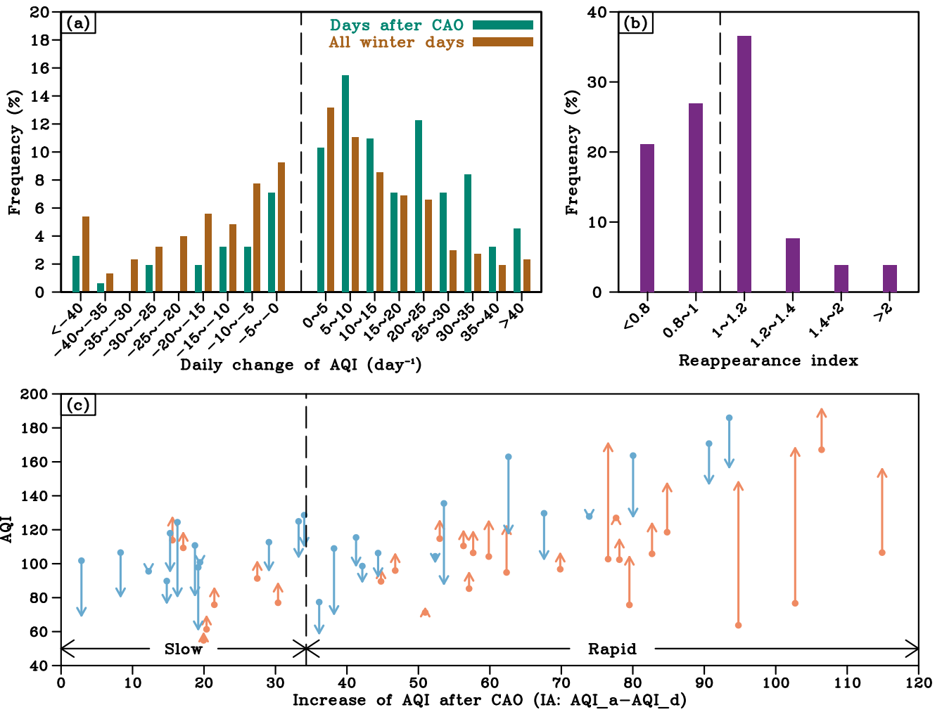
Figure 3: (a) Statistical distribution of daily change of AQI calculated by all of days during the 8 winters (brown bars) and days during the period after the CAOs (green bars). (b) Statistical distribution of the reappearance index of air pollution in 52 CAO events. (c) The increase in the AQI (x-axis) and the change in the AQI from the period before the CAO to the period after CAO (vertical arrows) in 52 CAO events. Black dashed line denotes the standard deviation of AQI. The arrowhead and tail represent AQI a and AQI b , respectively. The orange (blue) arrows denote that the AQI worsens (better) after CAO.
