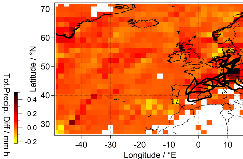
360 Figure 6. Average total precipitation difference between ERA5 and EMAC over Europe and North Atlantic (73 – 28 °N, -50 – 15°E; contains modified Copernicus Climate Change Service information; Hersbach et al. 2018). The North Atlantic region was included in view of the H 2 O 2 lifetime in the atmosphere and the air mass origins based on backward trajectories. The performed flights are indicated in black.
