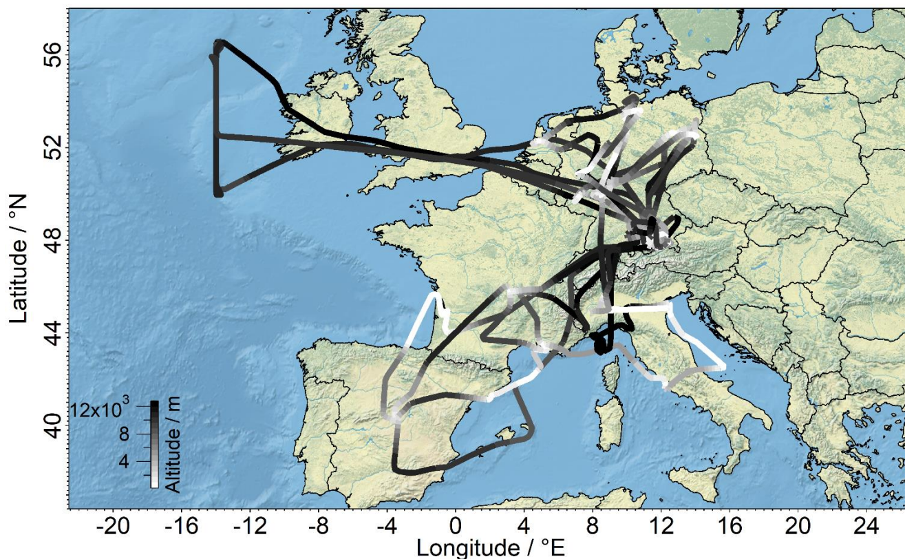
Figure 1. Flight tracks of the BLUESKY measurement campaign over Europe color-coded by GPS altitude. All flights were performed from the flight base in Oberpfaffenhofen, Germany (48 °N, 11 °E).
