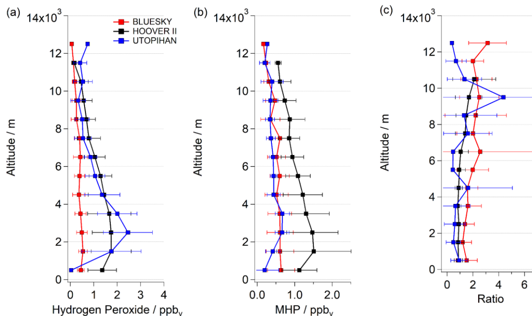
Figure 3. Comparison of vertical hydrogen peroxide profiles (a), MHP (b) and MHP/H 2 O 2 ratio (c) during BLUESKY (red) with outcomes of the earlier campaigns, HOOVER II (black) and UTOPIHAN-ACT II/III (blue). The data was plotted as mean ± 1 sigma.
