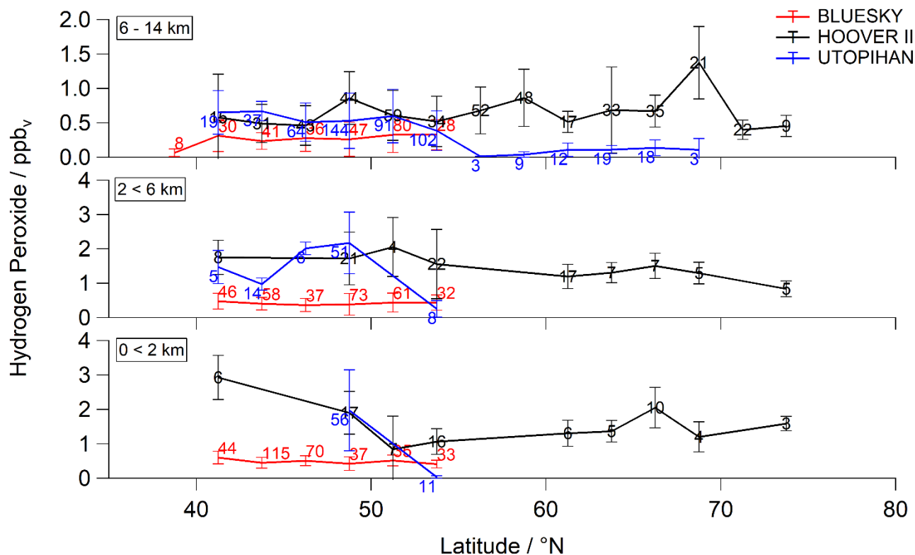
Figure 2. Latitudinal dependence of hydrogen peroxide concentrations (mean \pm 1 sigma) compared to former campaigns (red: BLUESKY; black: HOOVER II; blue: UTOPIHAN-ACT). The data with 2 min time resolution was subdivided into three atmospheric layers, upper troposphere, middle troposphere and boundary layer (from top to bottom) with mean values binned for 2.5° of latitude for each tropospheric layer. The corresponding numbers indicate the total amount of data points per bin.
