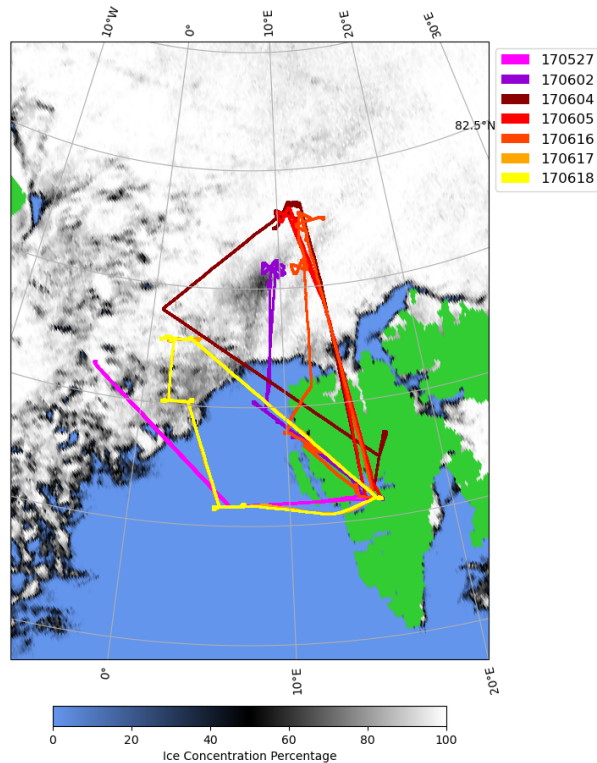
Figure 1. Flight paths for the ACLOUD flights with Polar 6 aircraft included in the analysis overlaid on pack ice extent as of 2 June. pack ice data is derived from measurements of the Advanced Microwave Scanning Radiometer 2 (AMSR2) at 89 GHz ( www.seaice.uni-bremen.de ; Spreen et al. (2008)).
