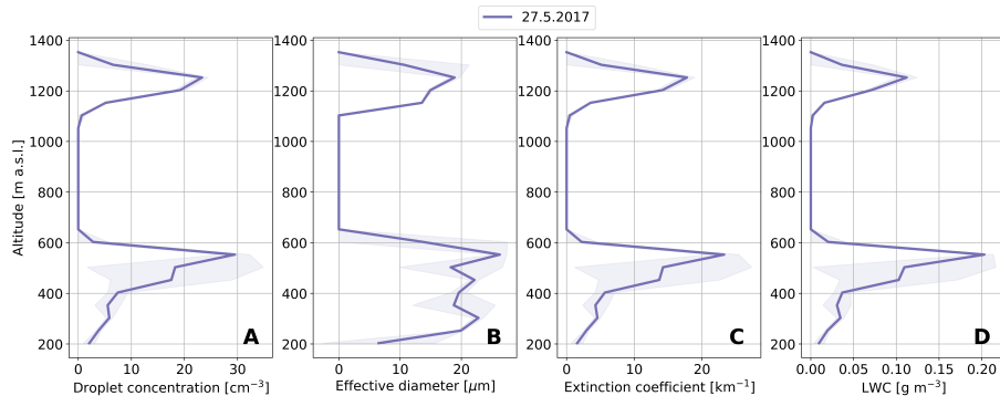
Figure 3. Vertical profile of average droplet concentration (A), droplet effective diameter (B), droplet extinction coefficient (C) and liquid water content (LWC) (D) performed on 27 May during the cold period. The 10-s average measurement data was binned in altitude bins with bin width of 49.3 m for calculating the statistics. The shaded area illustrates the standard deviations. The statistical uncertainty in droplet number concentration was below 0.3 \text{ cm}^{-3} . Cloud sampling was performed between 78.7^\circ\text{N} and 79.8^\circ\text{N} and 3.3^\circ\text{W} and 4.1^\circ\text{E} .
