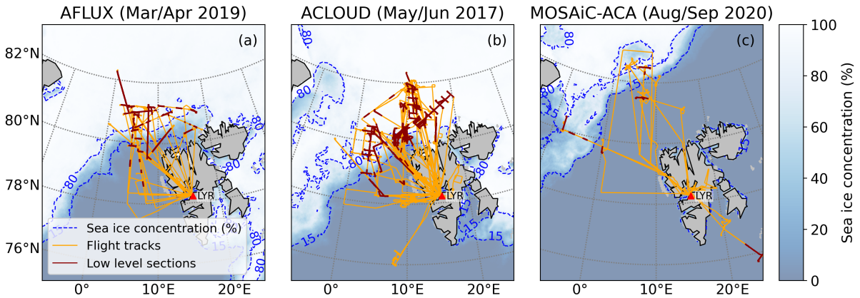
Figure 1. Flight tracks (red/orange) and low-level sections (bold brown/dark red) performed during (a) AFLUX, (b) ACLOUD, and (c) MOSAiC-ACA based at Longyearbyen (LYR). Each panel shows the mean sea ice concentration f_{ice} (derived from space-borne observations, Spreen et al., 2008) present during the respective campaign, the dashed blue lines indicate the 15 % and 80 % isolines of sea ice concentration f_{ice} that confine the MIZ according to the definition of Strong and Rigor (2013).
