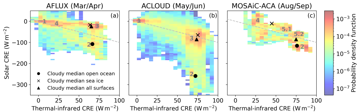
Figure 9. Two-dimensional probability density function of the solar CRE_{sol} and the TIR CRE_{TIR} for (a) AFLUX, (b) ACLOUD, and (c) MOSAiC-ACA. The diagonal dashed lines represent the 0 \text{ W m}^{-2} iseline of the total (i.e., the sum of the solar and TIR) CRE_{tot} . The symbols represent the median of CRE_{sol} and CRE_{TIR} over the surface types given in the legend in (a) and only considering cloudy observations (equivalent LWP > 5 \text{ g m}^{-2} ) median CREs over the different surface types. The numbered modes represent (1) cloud-free, (2) cloudy open ocean, (3) cloudy sea ice, (4) thin/broken clouds, and (5.1/5.2) cloudy MIZ conditions.
