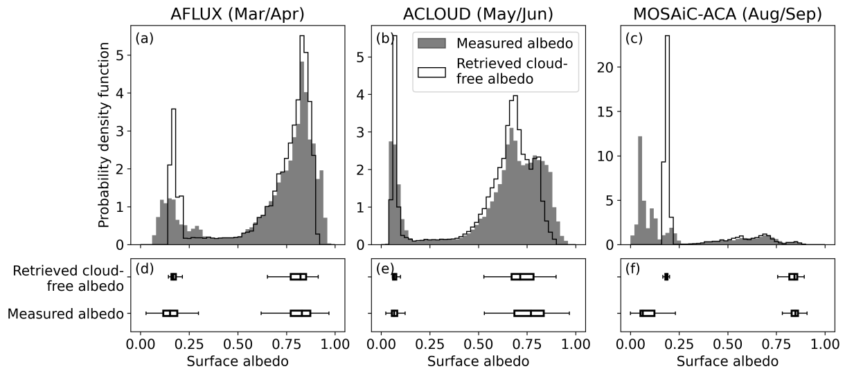
Figure 6. Probability density function of the surface albedos measured in mostly cloudy conditions (shadings) and retrieved for cloud-free conditions (lines) for (a) AFLUX, (b) ACLOUD, and (c) MOSAiC-ACA. (d–f) Box-whisker plots of the retrieved cloud-free and measured surface albedo separated for open ocean (left boxplots) and sea ice (right boxplots).
