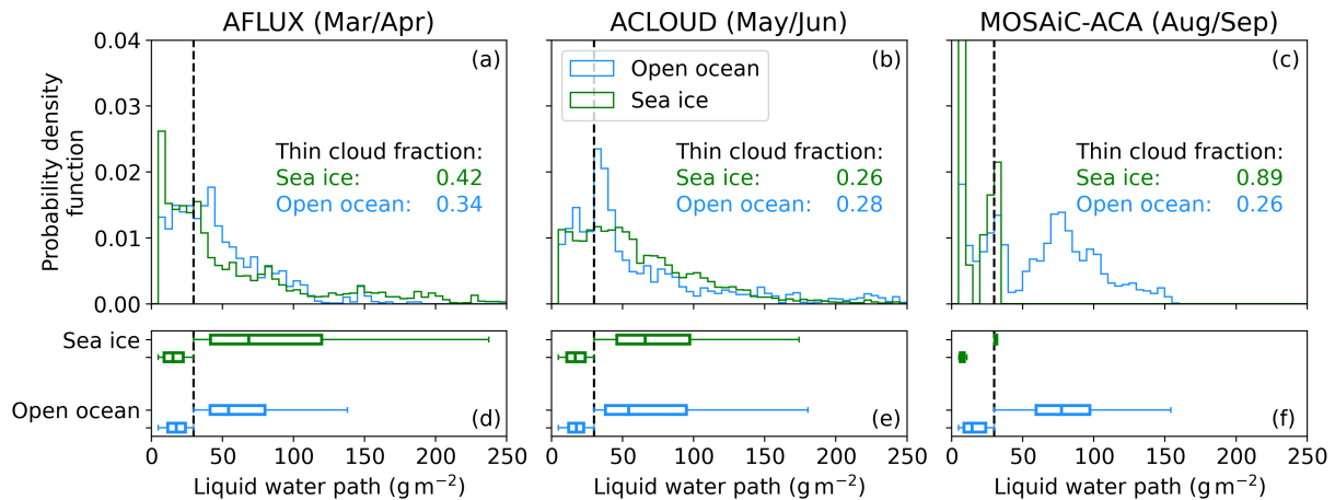
Figure 3. Probability density function of the equivalent LWP over sea ice and open ocean (colour-coded) for (a) AFLUX, (b) ACLOUD, and (c) MOSAiC-ACA. Only observations classified as cloudy (equivalent LWP > 5 \text{ g m}^{-2} ) were considered. The vertical dashed lines located at 30 \text{ g m}^{-2} indicate the threshold used for the separation of thin and thick clouds. The numbers in (a–c) represent the fraction of observations with thin clouds with respect to the total amount of cloudy observations. (d–f) Box-whisker plots of the equivalent LWP separating thin (left boxplots) and thick clouds (right boxplots).
