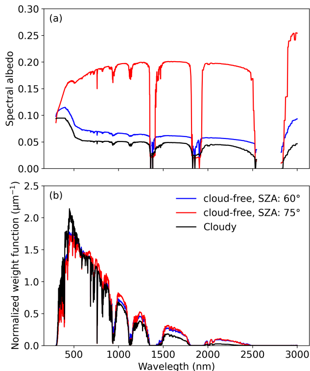
Figure 4. (a) Spectral Simulations of the spectral surface albedo \alpha_\lambda of open ocean for two different SZAs in cloud-free conditions, and for cloudy conditions (LWP of 80 \text{ g m}^{-2} , independent of SZA). (b) Spectral Simulations of the spectral normalized weight functions w for the same scenarios. The wind speed of 1 \text{ m s}^{-1} represents a calm surface.
