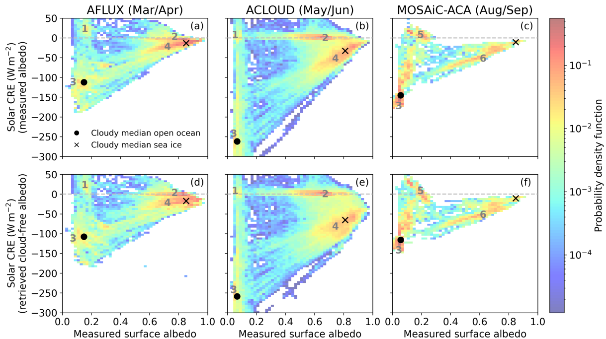
Figure 7. Two-dimensional probability density function of the solar CRE_{sol} and the measured (mostly cloudy) surface albedo (as an indicator for the surface type) for AFLUX (a,d), ALOUD (b,e), and MOSAiC-ACA (c,f). The upper row (a–c) shows the distributions of the solar CRE_{sol} neglecting the cloud-induced change of the surface albedo, while this effect is included in the lower row (d–f). The horizontal dashed lines mark a CRE_{sol} of 0 \text{ W m}^{-2} . The symbols represent the median of CRE_{sol} and the measured surface albedo over the surface types given in the legend in (a) and only considering cloudy observations (equivalent LWP > 5 \text{ g m}^{-2} ) median CRE_{sol} . The numbered modes represent (1) cloud-free open ocean, (2) cloud-free sea ice, (3) cloudy open ocean, (4) cloudy sea ice, (5) thin/broken clouds, and measured surface albedos over the different surface types (6) cloudy MIZ conditions.
