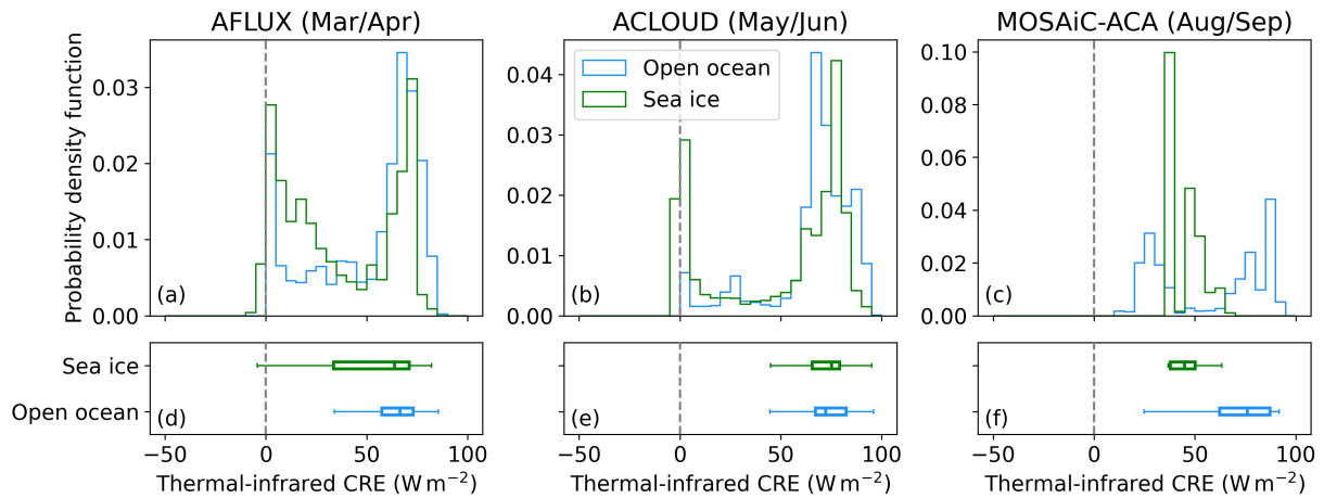
Figure 8. Probability density function of the \text{CRE}_{\text{TIR}} for (a) AFLUX, (b) ACLOUD, and (c) MOSAiC-ACA, separated for sea ice and open ocean (colour-coded). (d–f) Box-whisker plots of the \text{CRE}_{\text{TIR}} only considering cloudy observations (equivalent LWP > 5 \text{ g m}^{-2} ). The vertical dashed lines mark a \text{CRE}_{\text{TIR}} of 0 \text{ W m}^{-2} . Note that, due to a lack of the corresponding observations, none of the modes in (c) represents actual cloud-free conditions. The thinnest clouds, however, revealed an equivalent LWP < 5 \text{ g m}^{-2} and did, thus, not contribute to the statistics shown in (f).
