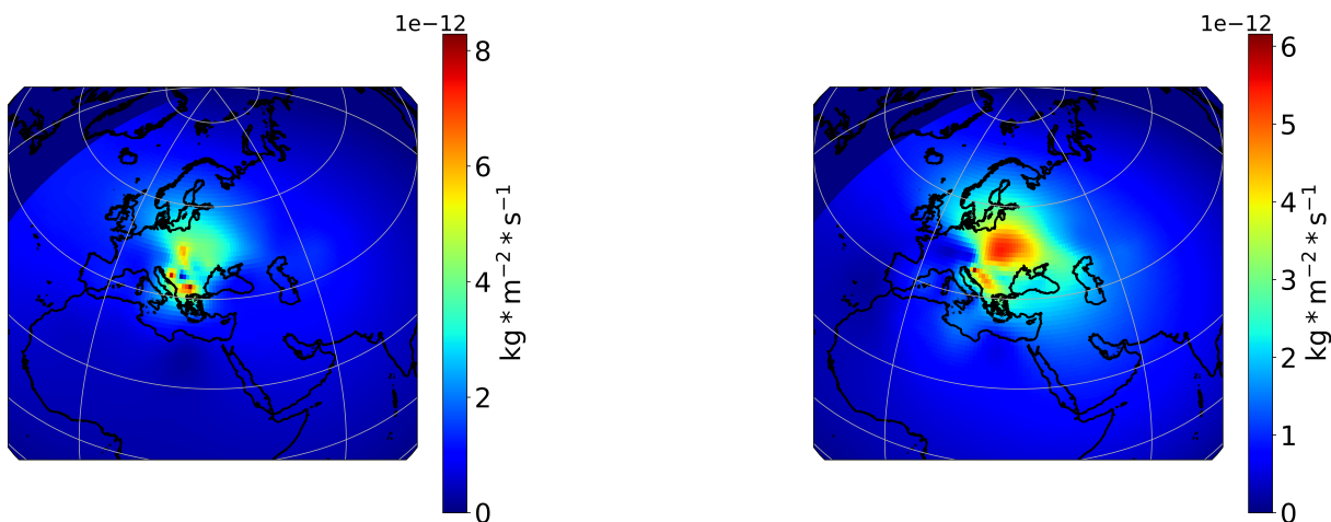
(a) Solution excluding data from Vilnius, Dushanbe, Kurchatov, Secondary Sulfate aerosol
