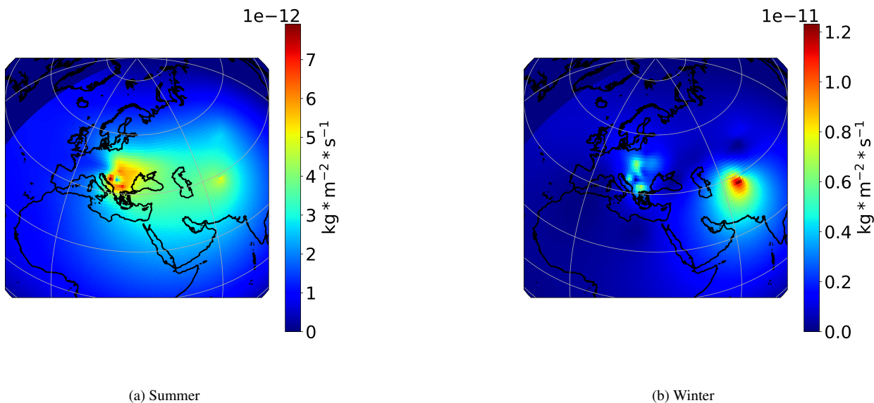
Figure A4. Tikhonov regularization for Secondary Sulfate for 14 stations, summer and winter
