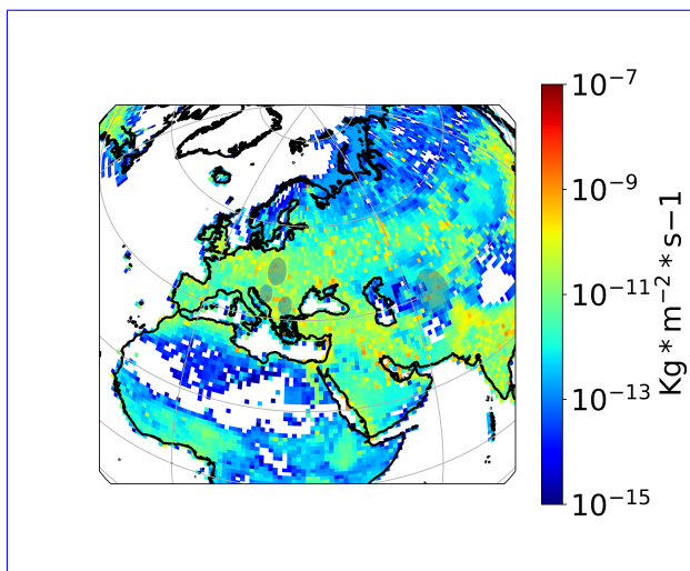
(c) OMI-HTAP EMISSIONS 2015 for SO_2
