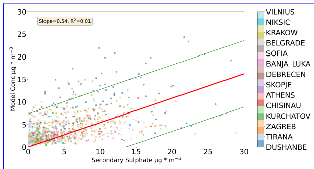
(a) Secondary Sulfate aerosol, solution for 14 cities, no intercept
