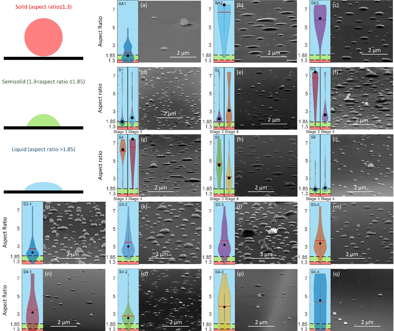
Figure 5. Violin plots of ‘corrected’ aspect ratio (left) and typical tilted images (right) of Pico 2014 (a to c), Pico 2015 1060 (d to i), and Pico 2017 (j to q). Distributions in the left panels of (d to i) are the aspect ratio of Pico 2015 particles collected on stages 3 (left) and 4 (right). The shaded region corresponds to the different phase states (red: solid state; green: semisolid state; blue: liquid state). The red lines indicate the means, and the black dots the medians.
