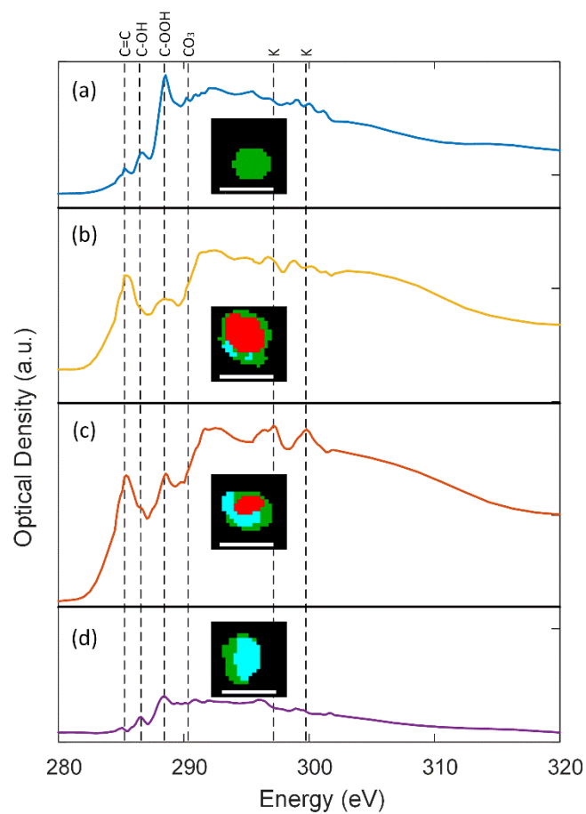
1055 Figure 4. Representative STXM-NEXAFS spectra of (a) organic particle (green), (b) EC core (red) coated by OC (green), (c) internally mixed elemental carbon (red), and IN (cyan) core coated by OC (green), and (d) IN (cyan) core coated by OC (green) from Pico 2017 S3-3 and S4-2 samples. White scale bars represent 500 nm.
