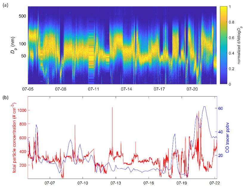
1045 Figure 2. (a) Normalized particle size distribution from 10 to 800 nm measured from SMPS measurements, and (b) SMPS derived total particle concentrations (left y-axis, red line) and CO tracer retrieved from FLEXPART simulations (right y-axis, blue line) from 05 to 21 July 2017.
