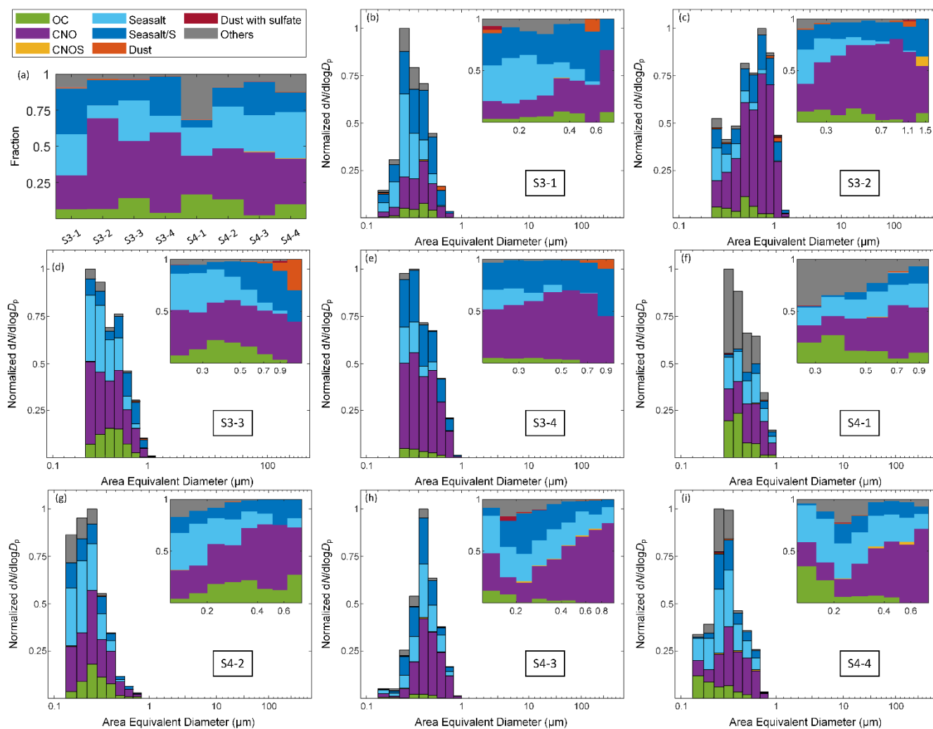
1050 Figure 3. Chemically-resolved size distributions were inferred from the CCSEM-EDX data for 2017. (a) Fraction of different particle types for all samples. Normalized chemically-resolved size distributions of (b) S3-1, (c) S3-2, (d) S3-3, (e) S3-4, (f) S4-1, (g) S4-2, (h) S4-3, and (i) S4-4. Inserts represent the normalized number fraction of different particle types as a function of particle size.
