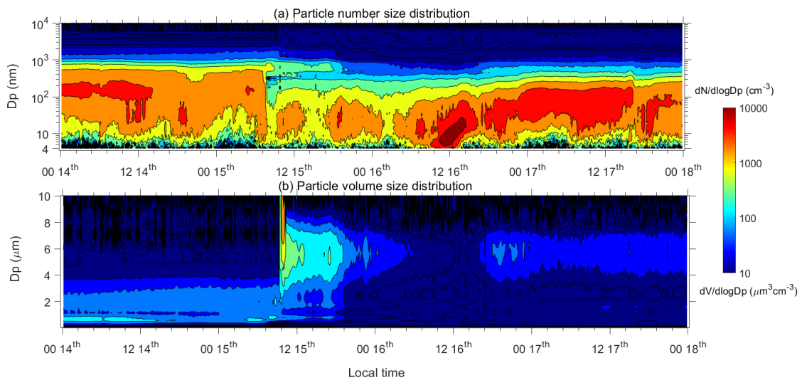
310 Fig. 7 Particle number (a) and volume (b) distributions on March 14–17, 2021, at CAMS station.
