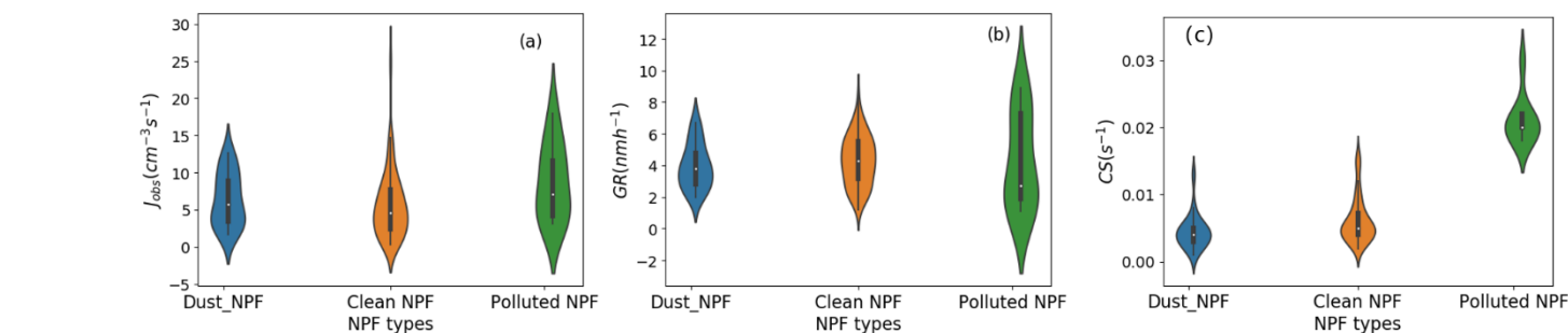
Fig. 4 The violin plot of formation rate ( J_{\text{obs}} ) (a), growth rate ( GR ) (b), and condensation sink ( CS ) of dust-related NPF (Dust_NPF) and other NPF events under clean (Clean NPF) and polluted conditions (Polluted NPF). The marker represents the median value; a box indicating the interquartile range, and the shaded area represents the distribution probability.
