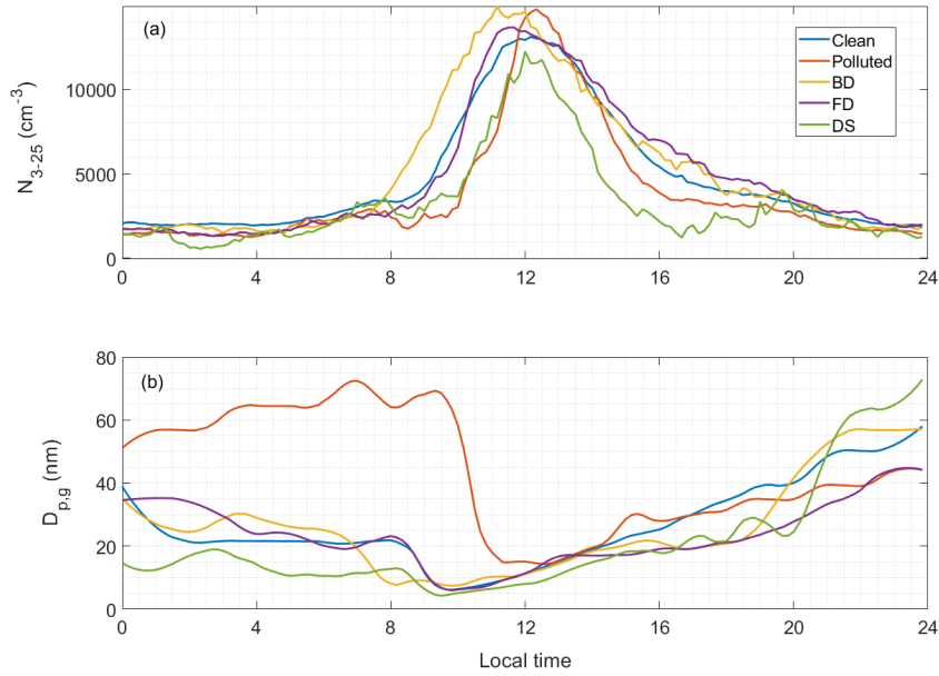
280 Fig. 5 the mean diurnal variation of number concentration of particles in the size range of 3-25 nm ( N_{3-25} ) (a) and geometric mean diameter ( D_{p,g} ) (b) of NPF events occurred under clean, polluted conditions and influenced by blowing dust (BD), floating dust (FD) and dust storm (DS), respectively.
