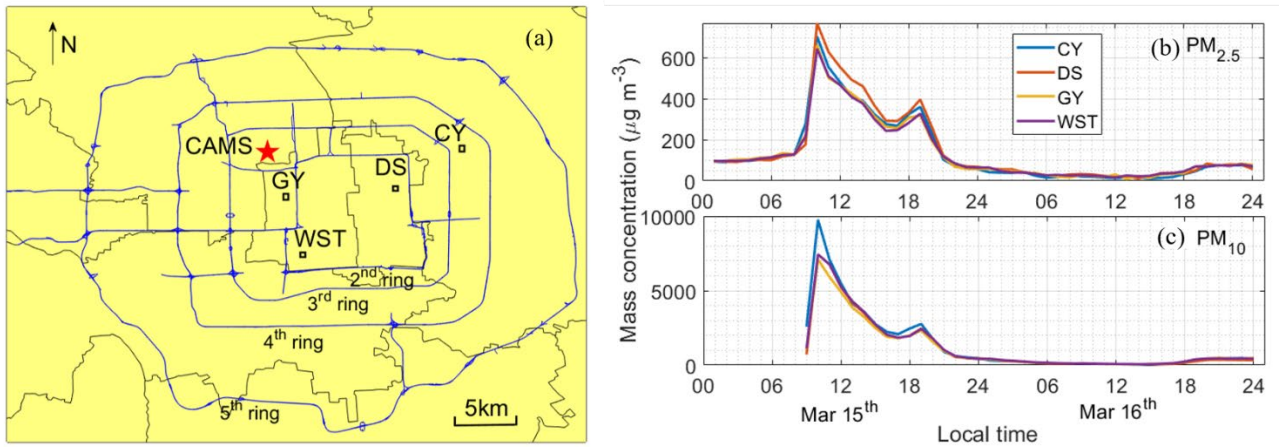
300 Fig. 6 The location map of CAMS site and four air quality monitoring sites, including Guanyuan (GY), Wanshou Temple (WST), Dongsì (DS), and Chaoyang (CY), in urban Beijing (a), as well as \text{PM}_{2.5} and \text{PM}_{10} mass concentration at each location (b).
