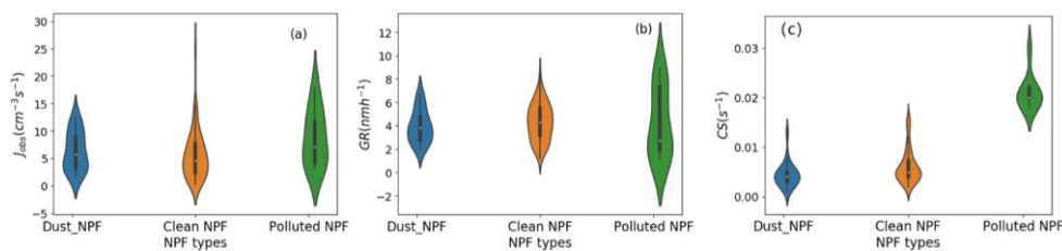
Fig. 4 The violin plot of formation rate ( J_{obs} ) (a), growth rate ( GR ) (b), and condensation sink ( CS ) of dust-related NPF (Dust_NPF) and other NPF events under clean (Clean NPF) and polluted conditions (Polluted NPF). The marker represents the median value; a box indicating the interquartile range, and the shaded area represents the distribution probability.
