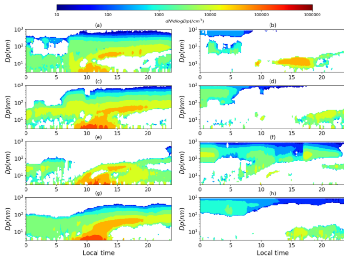
Fig. 3-2 The positive (a, c, e, g) and negative (b, d, f, h) anomalies of PNSD derived by the mean PNSDs of NPF events on non-dust days in spring (March, April, and May) subtracting the means of dust-related NPF days in 2017 (a, b), 2018 (c, d), 2019 (e, f) and 2021 (g, h).
