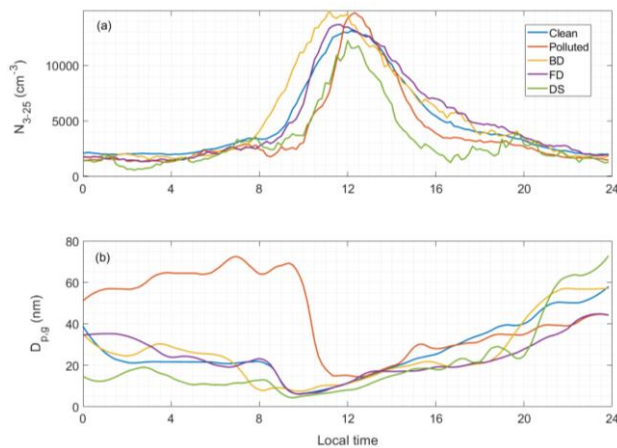
Fig. 5. the mean diurnal variation of number concentration of particles in the size range of 3-25 nm ( N_{3-25} ) (a) and geometric mean diameter ( D_{p,g} ) (b) of NPF events occurred under clean, polluted conditions and influenced by blowing dust (BD), floating dust (FD) and dust storm (DS), respectively.
