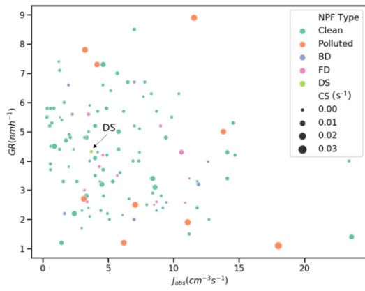
Fig. 3. Scatter plot of formation rate ( J_{obs} ), grow rate ( GR ) and condensation sink ( CS ) as categorized by different NPF event types, including the cases occurring under clean, polluted conditions and influenced by blowing dust (BD), floating dust (FD) and dust storm (DS).
