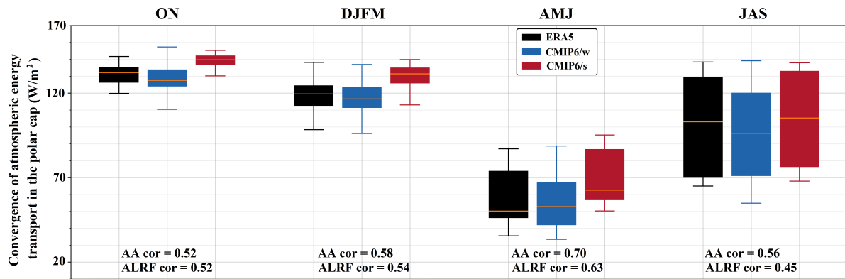
Figure 8. a) Seasonal Pan-Arctic atmospheric energy transport convergence north of 66° N, obtained from ERA5, and the model subsets CMIP6/w and CMIP6/s, respectively, during 2000–2014. The seasonal inter-model correlation coefficients between the seasonal mean of transport term and historical AA / ALRF (including all models in Table 1 with daily resolution ) are given in the lower part of each panel. b) Mean Wasserstein distance (WSD) between ERA5 transport patterns and the corresponding CMIP6 patterns for CMIP6/w and CMIP6/s subsets, respectively. The WSD for individual CMIP6/w and CMIP6/s models are shown by transparent crosses. The seasonal inter-model correlation coefficients between WSD and AA / ALRF are given in the lower part of each panel. Correlation coefficients that are statistically significant are marked in bold. We use daily-monthly output data for both ERA5 and CMIP6 in this analysis. Details on the data processing derivation of atmospheric energy transport convergence are given in Section 2.6.
