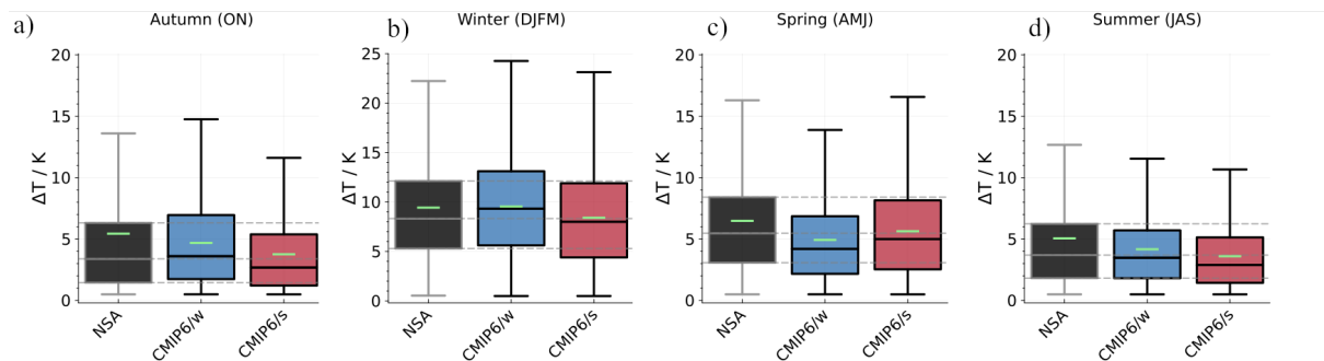
Figure 5. Seasonal inversion strengths \Delta T as box plots, obtained from radio soundings at the North Slope of Alaska (NSA) in Utqiaġvik, Alaska, USA, and from the model subsets CMIP6/w and CMIP6/s, respectively. The box plots correspond to Fig. 4b showing the seasonal distribution of \Delta T from radio soundings during the MOSAiC expedition. NSA data was collected during 2003–2014, and is compared to co-located 6-hourly model data in the period of 2010–2014. Details on the data processing are given in Section 2.3.
