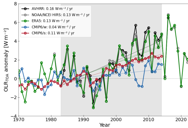
Figure 9. Time series of net outgoing long-wave radiation at TOA (all-sky) OLR_{TOA} anomaly with respect to 1983–1997 for AHRR satellite retrievals , NOAA/NCEI HIRS and ERA5 climate data records , just as the model subsets CMIP6/w and CMIP6/s, respectively. Trends are derived for both satellite observations / reanalysis, and model subsets as linear fit between 1982 and 2014, from the beginning of the satellite record to the end of for the historical CMIP6 simulations data overlap period (1983–2014; shaded area) . The fluxes are averaged over the Arctic area north of 66^\circ N , and account for the extended winter period DJFM. For the comparison, we use the collection of monthly-mean model diagnostics. Details on the data processing are given in Section 2.7.
