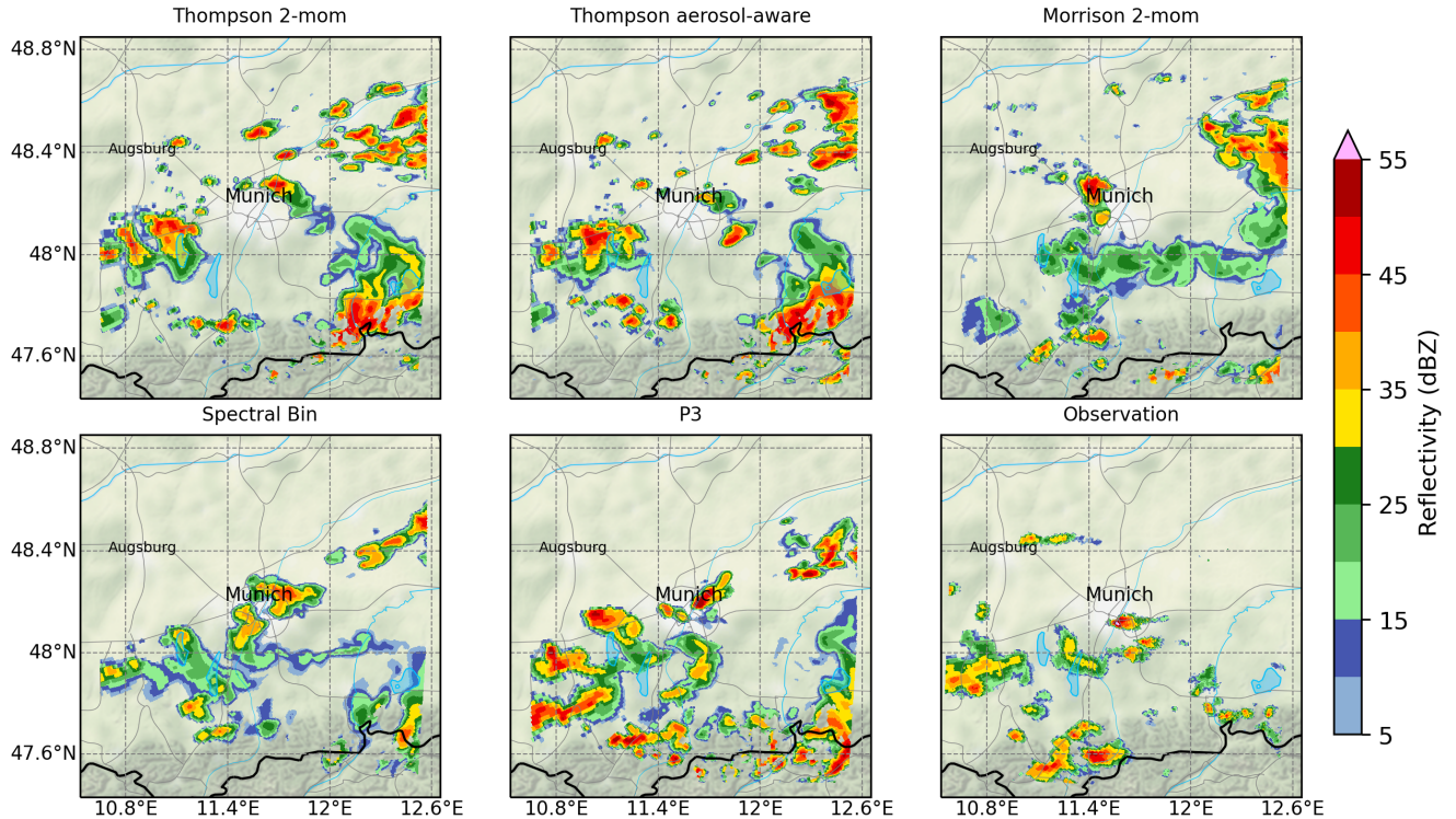
Figure 1. Simulated and measured reflectivity at July 7th, 2019, 12:45 UTC over the full domain size with a grid spacing of 400 m. Simulated reflectivity from the WRF model output after applying the CR-SIM forward simulator Oue et al. (2020). Background map tiles by Stamen Design (Stamen Design, 2022). Background map data by OpenStreetMap (OpenStreetMap, 2022, © OpenStreetMap contributors 2022. Distributed under the Open Data Commons Open Database License (ODbL) v1.0.). Roads, rivers, and lakes made with Natural Earth (Natural Earth, 2022).
