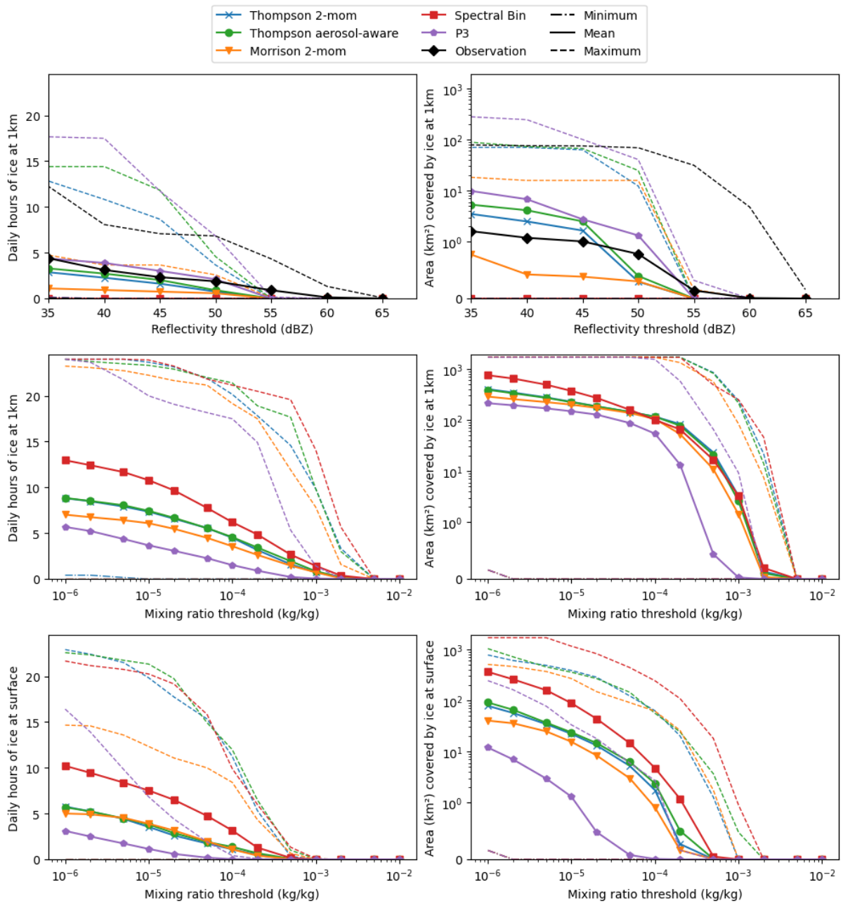
Figure 5. Same as Fig. 3, but for hail and graupel ice statistics. Frequency (left column) and area (right column) of hail/graupel ice events above various thresholds. Minimum (dashed-dotted line), mean (solid line), and maximum (dashed line) over the 30-day data set. First row: statistics based on simulated and observed reflectivity thresholds at 1 km altitude. Simulated reflectivity from WRF model output after applying the CR-SIM forward simulator Que et al. (2020) ( Que et al., 2020 ). Second row: statistics based on mixing ratio thresholds at 1 km altitude. Third row: statistics based on thresholds for mixing ratio at the surface. Graupel mixing ratio is direct WRF model output. In case of The y-axis on the P3 scheme, rime ice mass mixing ratio right side is used instead of graupel mass mixing ratio logarithmically scaled, except for a small range around zero (0-1) with a linear scale.
