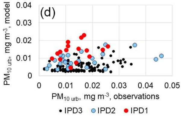
990 Figure 11: The relationship between model and measured urban aerosol optical depth at 550 nm ( AOD_{urb} - a,c) and urban component of PM_{10} ( PM_{10,urb} , in mg\ m^{-3} - b,d) for all cases ( n=229 ) (a,b) and for the cases without the effects of urban air advection from Moscow to Zvenigorod ( n=203 ) (c,d) at different IPD conditions. For consistency reason we show only quasi-simultaneous AOD and PM_{10} measurements during the daytime period with AOD observations. The cases affected by biomass burning aerosol were excluded. 2018.
