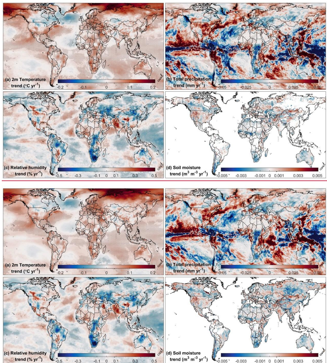
Figure 9. Global trends in temperature, total precipitation, relative humidity (1000 hpa) and soil moisture from 2001 to 2019. The "*" in the figure represents that the trend has passed the 95% significance test.
