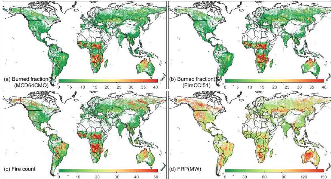
840 Figure 2. The spatial distribution of global fire burned fraction (BF), fire count (FC) and fire radiation power (FRP) from 2001 to 2019.
