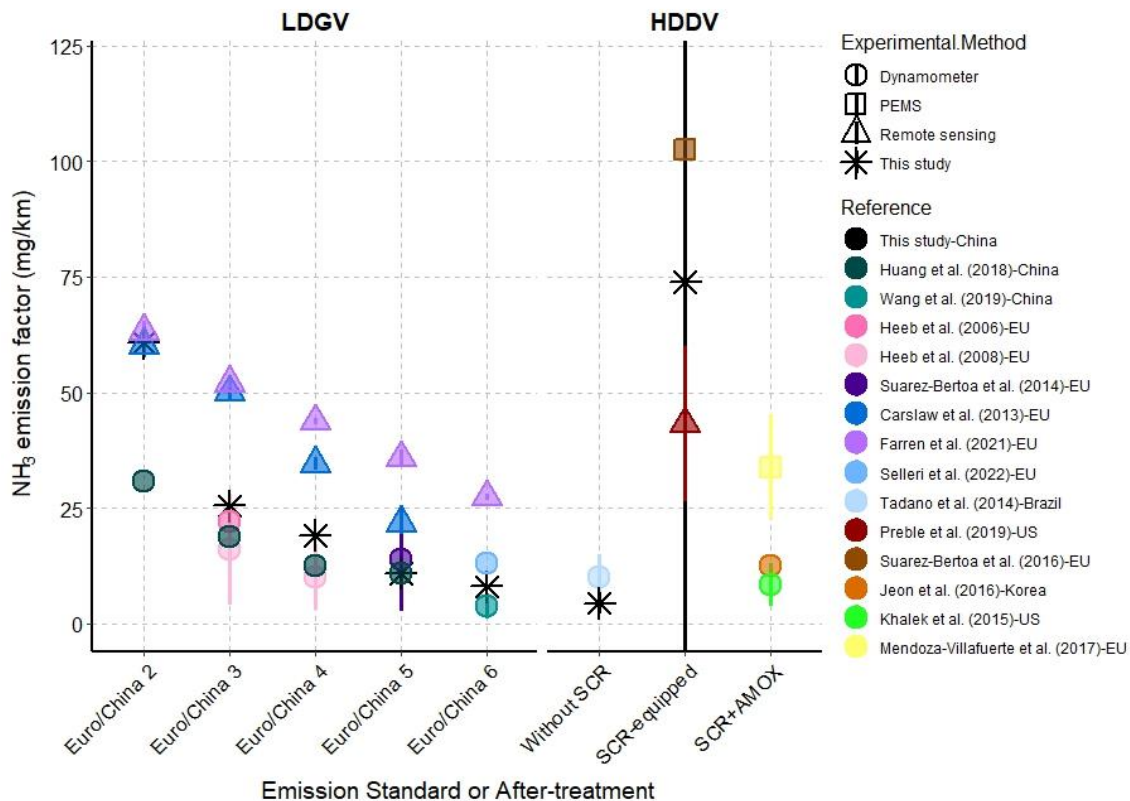
275 Figure 1: Comparison of distance-based NH 3 EFs for of LDGVs and HDDVs in this study and other relative studies, disaggregated by emission standard or after-treatment technology.
