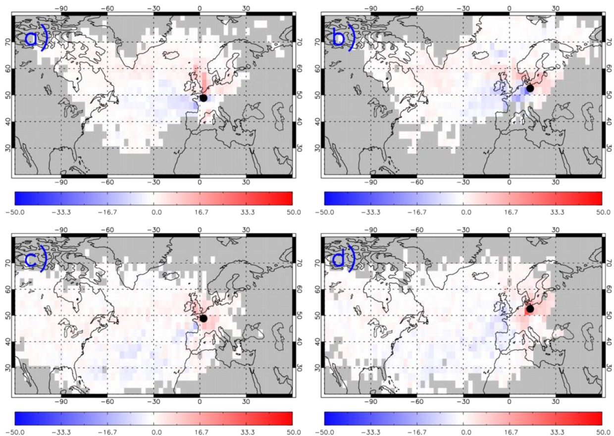
Figure R1: The May-August 2018-2017 difference between grid box trajectory point frequencies (as a percentage) for a) Paris surface, b) Berlin surface, c) Paris 500 hPa and d) Berlin 500 hPa.
