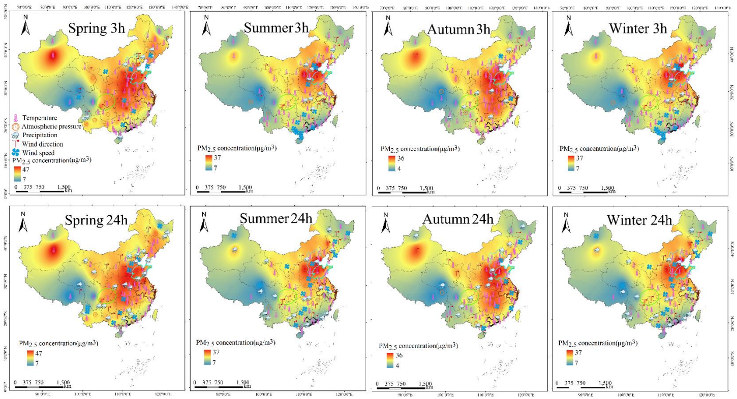
465 Figure 3: The dominant meteorological factor for PM 2.5 concentrations across China at 3h and 24h scale.
