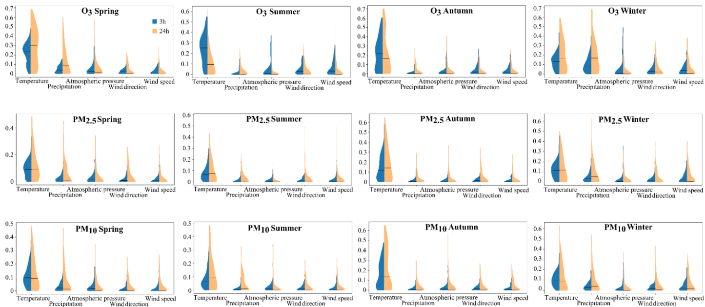
445 Figure 1: The violin chart of the \rho value of individual meteorological factors on PM 2.5 , PM 10 and O 3 across China at 3h and 24h scale.
