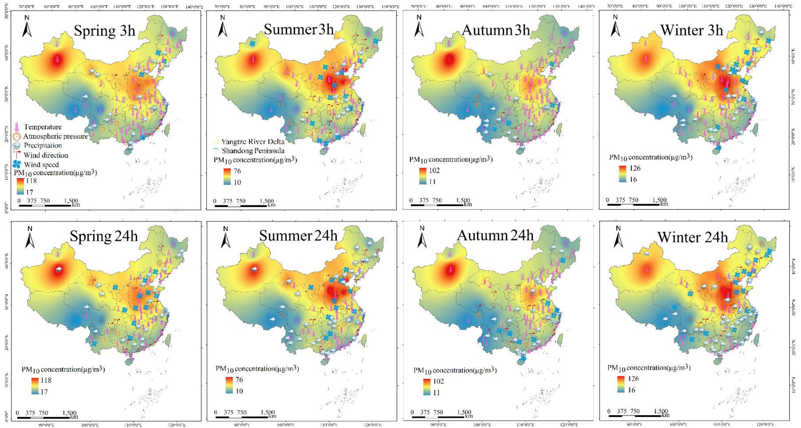
385 Figure 4: The dominant meteorological factor for PM 10 concentrations across China at 3h and 24h scale.
