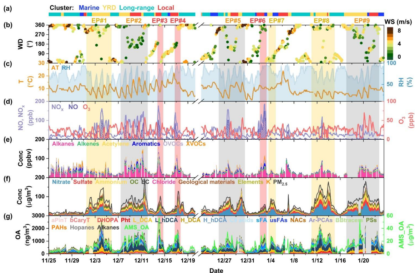
185 Figure 1. Time series of (a) air mass clusters; (b) wind direction (WD), wind speed (WS); (c) temperature (T), relative humidity (RH); (d) NO, NO x , O 3 ; (e) VOCs measured by GC-MS (see Table S2 for the VOC groups and individual VOCs); (f) major components of PM 2.5 and total PM 2.5 (dark line); and (g) organic molecular groups in PM 2.5 measured by TAG and total OA (green line) in PM 1 measured by AMS during the campaign. The concentration of geological materials was calculated to be 2.49[\text{Si}] + 1.63[\text{Ca}] + 2.42[\text{Fe}] , and concentration of elements was calculated as the sum of V, Cr, Mn, Ni, Cu, Zn, As, Se, Ba, and Pb. The nine episodic events were shaded in yellow, grey and 190 red, representing transport, mixed-influence and local episodes, respectively.
