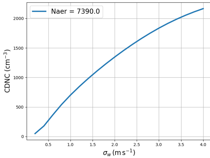
Figure B: Dependence between CDNC and the standard deviation of vertical velocity with measured aerosol size distribution from 19th May, 2018 based on a box model calculation using parameterized cloud droplet activation by Abdul-Razzak and Ghan (2000, https://doi.org/10.1029/1999JD901161 ).
