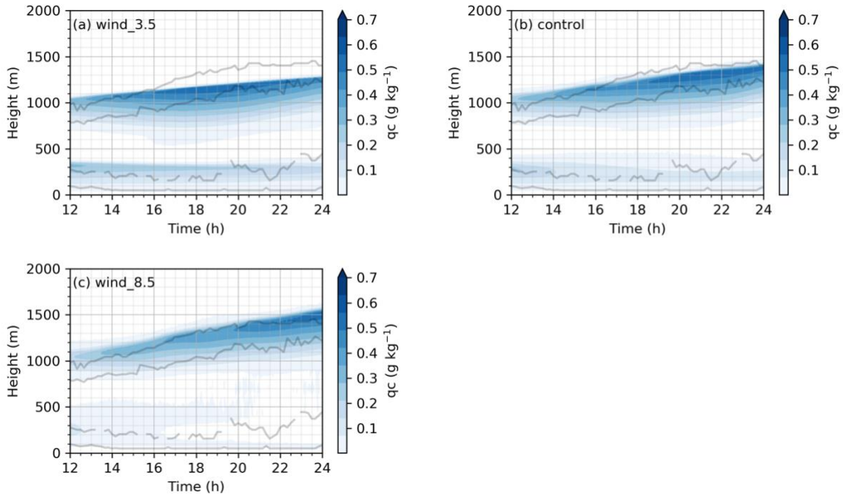
Figure 15. Model-domain average cloud droplet mixing ratio simulated with a: (a) U=3.5 \text{ m s}^{-1} (wind_3.5); (b) U=5.7 \text{ m s}^{-1} (control simulation) and (c) U=8.5 \text{ m s}^{-1} (wind_8.5). The two pairs of lines show the analyzed cloud base and cloud tops using both radar and lidar data. The first 3 hours are excluded as they are considered to be a spin-up period.
