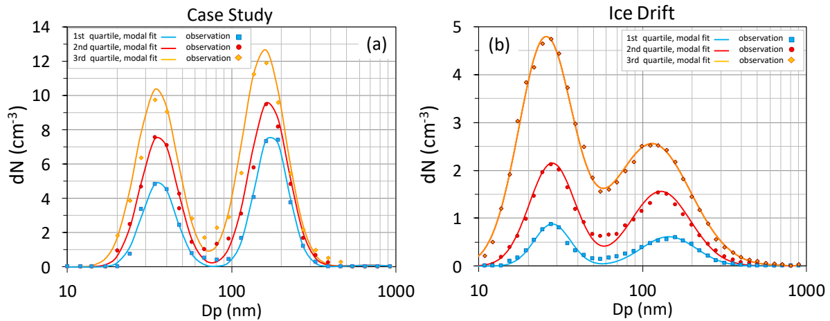
Figure 5. Aerosol number size distribution statistics (particle concentration in each size bin, dN vs. aerosol diameter, D_p ) shown for (a) the simulated case study (12:00 to 24:00 UTC on 18 August) and (b) the whole ice drift period (14 August - 14 September).
