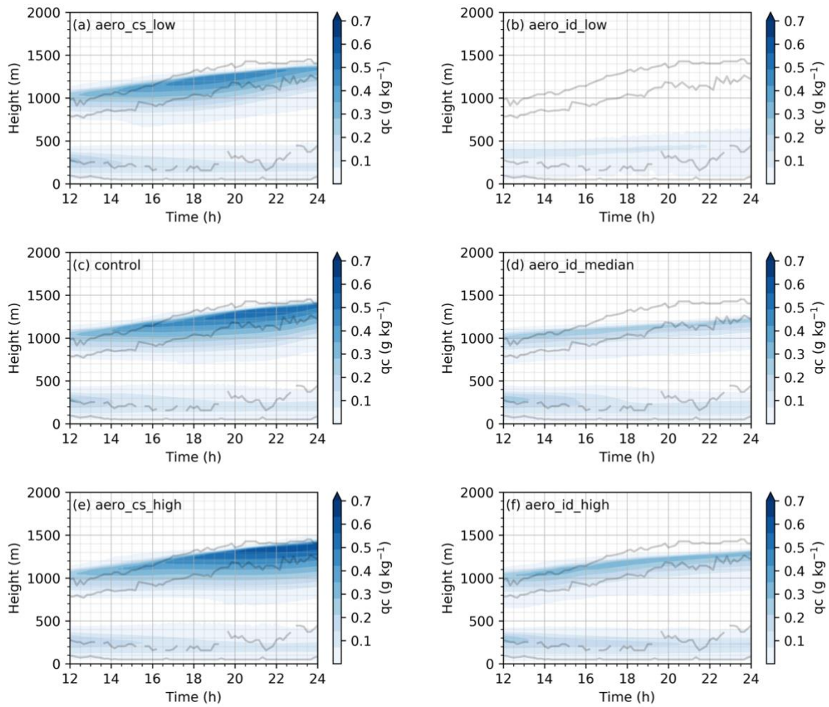
475 Figure 9. Model-domain average cloud droplet mixing ratio from: (left) aero_cs_low , control , aero_cs_high simulations, and (right) aero_id_low , aero_id_median , aero_id_high simulations (see Table 1 for simulation names). The two pairs of lines show the analyzed cloud base and cloud tops using both radar and lidar data. The first 3 hours are excluded as they are considered to be a spin-up period.
