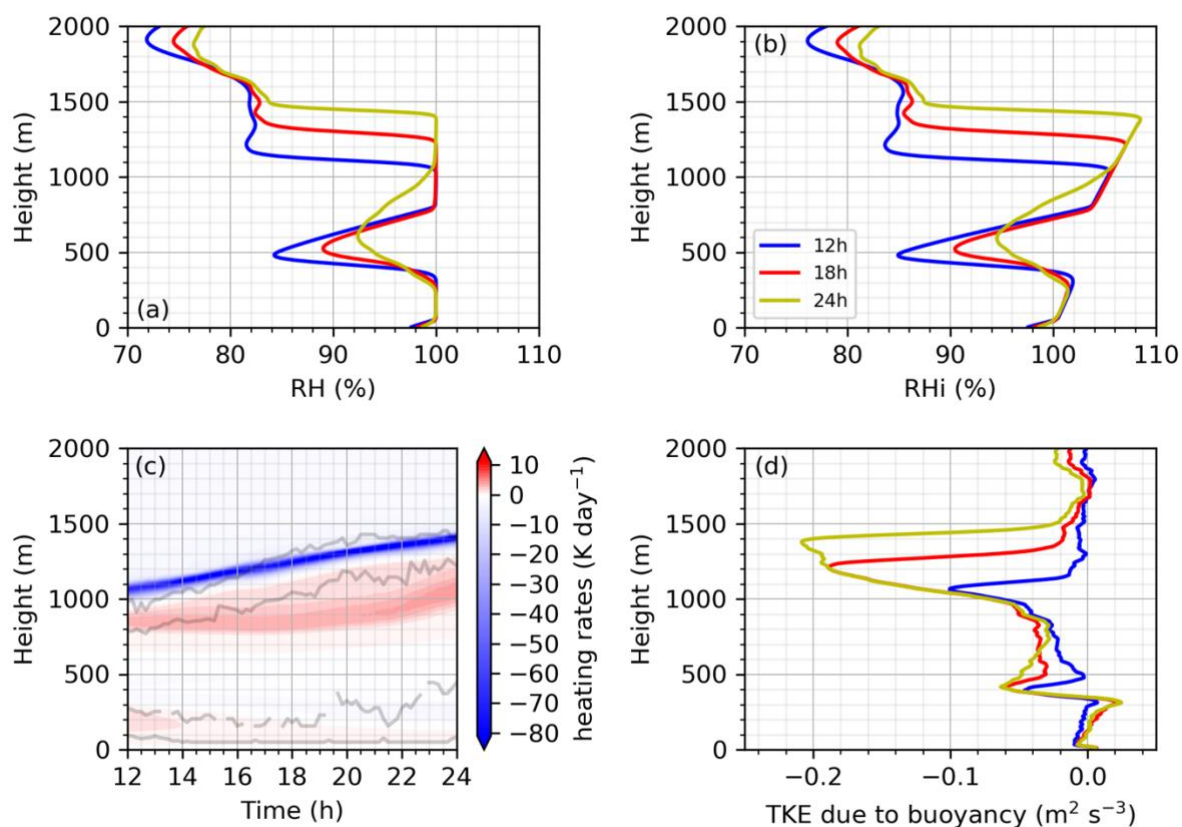
Figure A1. Simulated vertical profiles of (a) relative humidity, (b) relative humidity with respect to ice. (c) Model-domain average simulated vertical distribution of heating rates and (d) simulated vertical profiles of buoyancy induced turbulent kinetic energy (TKE). Note that simulated profiles are horizontal averages over the model domain.
