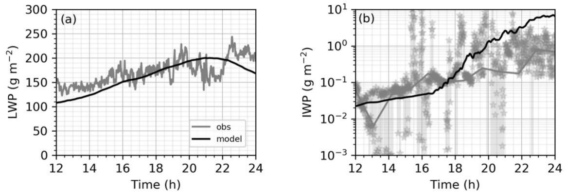
Figure 7. Model-domain average simulated and retrieved time series of: (a) total (liquid+rain) LWP and (b) total (ice+snow+graupel) IWP. Raw IWP is shown with a star symbol while the grey line represents the IWP 1h average. The first 3 hours are excluded as they are considered to be a spin-up period.
