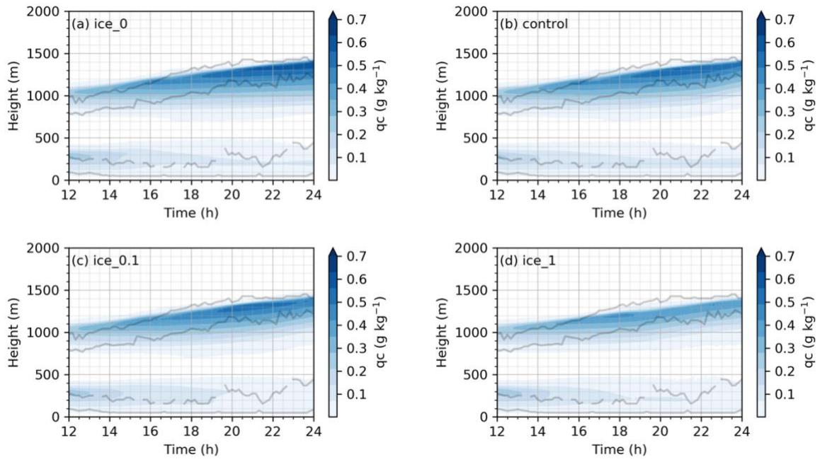
Figure 11. Model-domain average cloud droplet mixing ratio simulated with a: (a) no ice (ice_0); (b) the ice crystal number concentration = 0.01 \text{ L}^{-1} (control simulation); (c) the ice crystal number concentration = 0.1 \text{ L}^{-1} (ice_0.1); (d) the ice crystal number concentration = 1 \text{ L}^{-1} (ice_1). The two pairs of lines show the analyzed cloud base and cloud tops using both radar and lidar data. The first 3 hours are excluded as they are considered to be a spin-up period.
