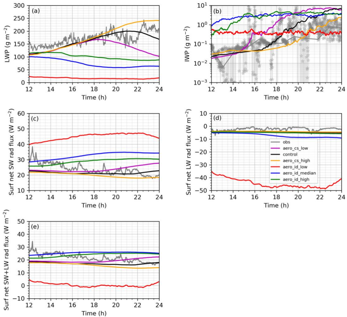
Figure 10. Model-domain averaged and retrieved time series of: (a) LWP, (b) IWP, (c) surface net shortwave (SW) radiative flux, (d) surface net longwave (LW) radiative flux and (e) surface net SW+LW radiative flux. The results from different sensitivity tests are in different colors (see the figure legend). The retrieved values from observations (obs) are in grey color. Raw IWP is shown with a star symbol while the grey line represents the IWP 1h average. The first 3 hours are excluded as they are considered to be a spin-up period.
