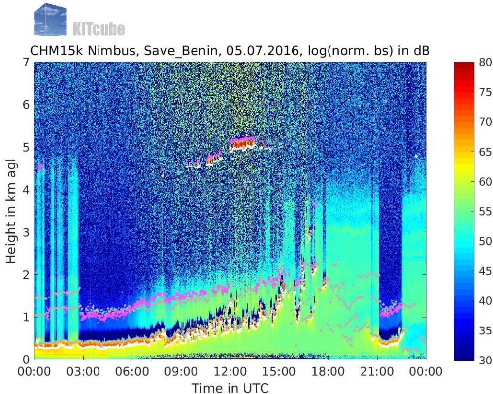
Figure 2: Ceilometer retrieval from the KITcube station in Savé, Benin from 5 July 2016. The retrieval shows the evolution of low-level clouds, starting from a nightly stratiform cloud deck that lifts after sunrise, broadens and breaks up around noon. Similarly to the insitu cloud measurements from the aircraft clouds are found on similar altitudes. Credits: N. Kalthoff
