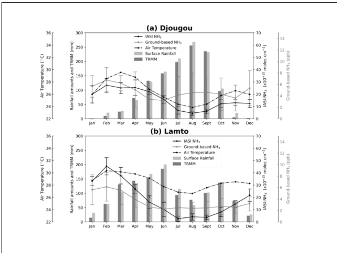
355 Figure 5. Mean monthly ground-based NH 3 concentrations (Djougou : 2005-2018 & Lamto : 1998–2018), IASI NH 3 total column densities (2008–2018), rainfall amounts, air temperatures measured by ground-based instruments (1998-2018) and TRMM (2005-2018) (Djougou : 2005-2018 & Lamto : 1998–2018) at (a) Djougou, Benin and (b) Lamto, Côte d'Ivoire. Error bars represent the mean absolute deviation.
