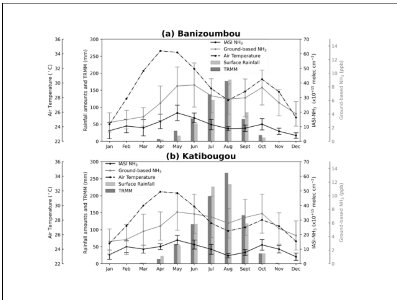
265 Figure 3. Mean monthly ground-based \text{NH}_3 concentrations (1998–2018), IASI \text{NH}_3 total column densities (2008–2018), rainfall amounts, air temperatures (1998-2018) measured by ground-based instruments (1998-2018) and TRMM (2005-2018) at (a) Banizoumbou, Niger and (b) Katibougou, Mali. Error bars represent the mean absolute deviation.
