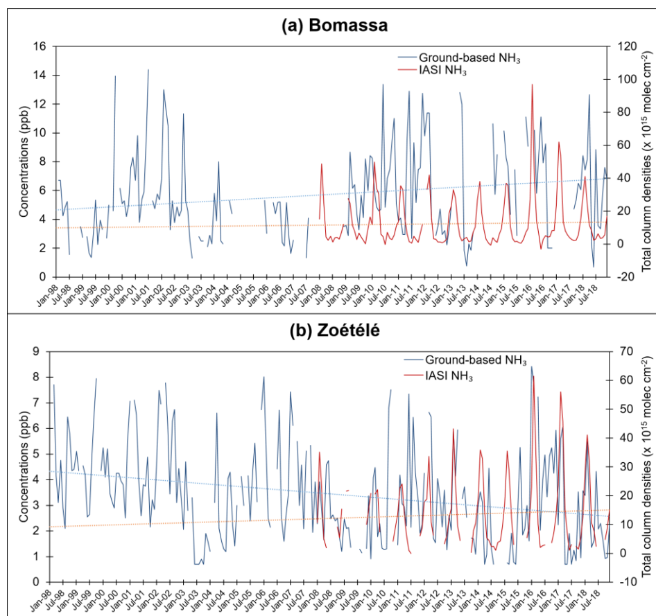
380 Figure 6. Monthly time-series of ground-based NH 3 concentrations over the period 1998–2018, IASI NH 3 total column densities from 2008 to 2018 at (a) Bomassa, Republic of Congo and (b) Zoétélé, Cameroon. The dashed lines represent the linear regression lines.
