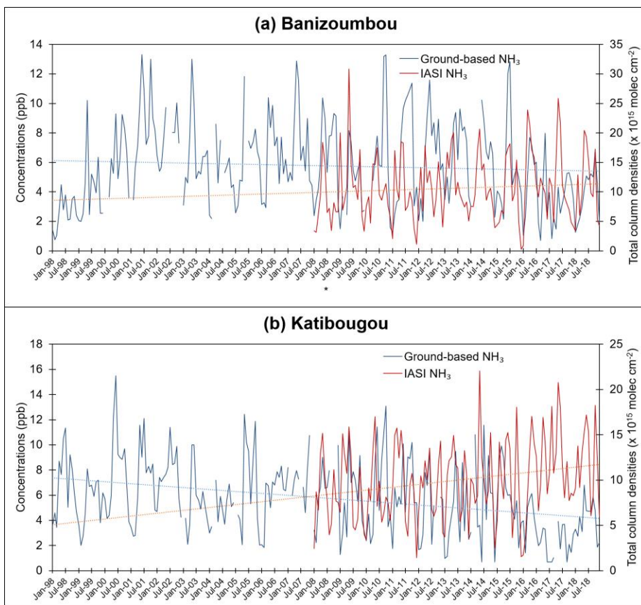
Figure 2. Monthly time-series of ground-based NH 3 concentrations over the period 1998–2018, IASI NH 3 total column densities from 2008 to 2018 at (a) Banizoumbou, Niger and (b) Katibougou, Mali. The dashed lines represent the linear regression lines.
