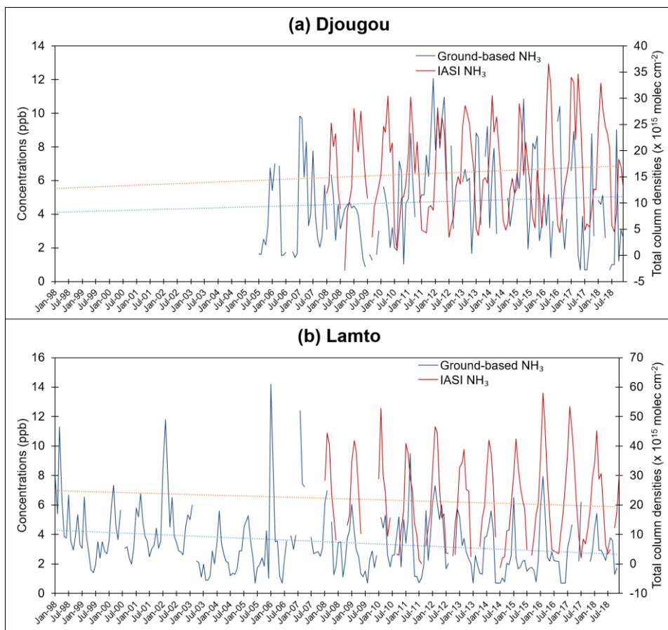
Figure 4. Monthly time-series of ground-based \text{NH}_3 concentrations over the periods 2005-2018 and 1998-2018, IASI \text{NH}_3 total column densities from 2008 to 2018 at (a) Djougou, Benin and (b) Lamto, Côte d'Ivoire. The dashed lines represent the linear regression lines.
