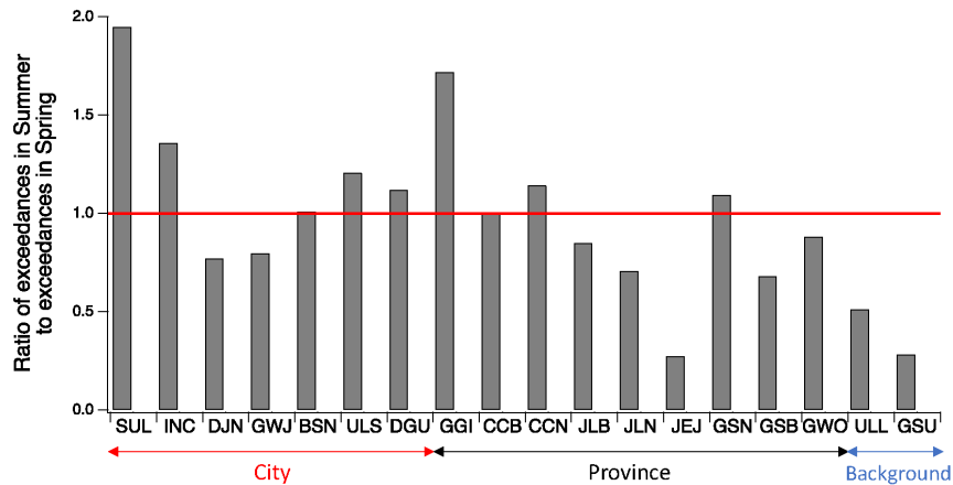
Figure 4. Ratio of O 3 exceedances in summer to exceedances in spring. The exceedances are defined as the fraction of the data with hourly ozone concentration greater than 70 ppb among all available data. The red line indicates an one to one line. X-axis denotes names of cities, provinces, and background sites. Cities – SUL (Seoul), INC (Incheon), DJN (Daejeon), GWJ (Gwangju), BSN (Busan), ULS (Ulsan), DGU (Daegu); Provinces - GGI (Gyeonggi-do), CCB (Chungcheongbuk-do), CCN (Chungcheongnam-do), JLB (Jeollabuk-do), JLN (Jeollanam-do), JEJ (Jeju Island), GSN (Gyeongsangnam-do), GSB (Gyeongsangbuk-do), GWO (Gangwon-do); Background sites - ULL (Ulleung Island), and GSU (Gosung, Gangwon-do). The data for 2002-2019 are utilized.
