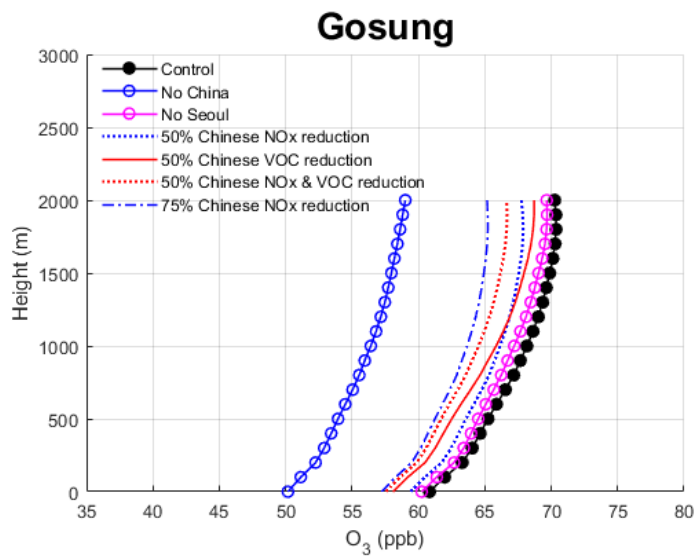
1 2 Figure 11. Vertical profiles of ozone from the WRF-Chem model simulations based on 3 various emission scenarios: (top) Seoul, and (bottom) Gosung, Gangwon-do. The model 4 results from 10 LT to 20 LT are averaged. 5
