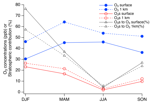
Figure 6. The contribution of stratospheric O 3 (O 3s ) to the O 3 concentrations in each season at surface and 1 km above ground level in South Korea. The plotted values are extracted from the CESMv2.2 results for the entire country.
