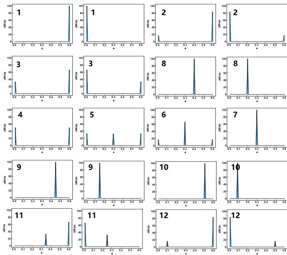
Figure S3. \kappa -PDFs for the 12 populations in the mixing state diagram.
