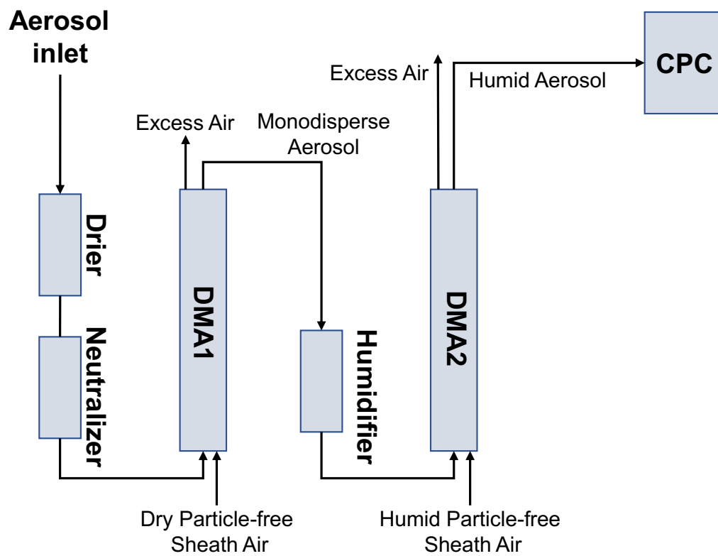
Figure S2. Schematic structure of the HTDMA
