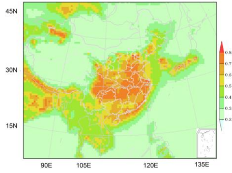
Figure 1. The ensemble spread of \lambda_{t,t}^a , at model level 1 in January 2016, when \beta=80 .
