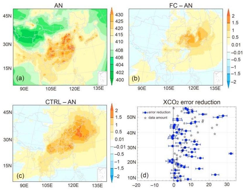
1195 Figure 87. The annual-averaged horizontal distribution of CO 2 concentrations (unit: ppm) near the surface in 2016: (a) AN: the analysis concentration; (b) FC-AN: the difference between the a posteriori flux simulation and analysis concentration fields; (c) CTRL-AN: the difference between the a priori flux simulation and analysis concentration fields; (d) the XCO 2 error reduction [see text for calculation; blue, with the standard deviation ( \pm ) of the analysis XCO 2 provided] and independent XCO 2 data amount (black stars, rescaled to 1:10) over 8°–57°N and 105°–120°E at different latitudes.
