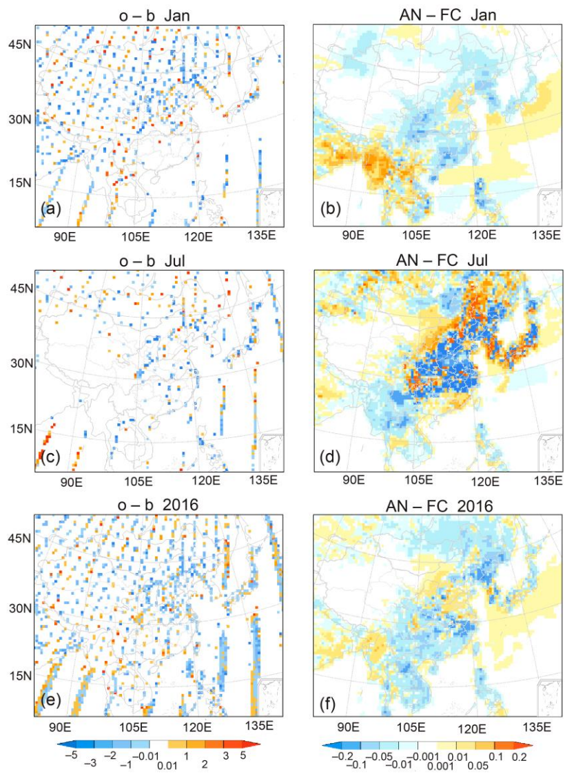
Figure 24. Observation increments (XCO 2 ; unit: ppm) and analysis increments (biosphere flux; unit: μmole m -2 s -1 ) in (a, b) January, (c, d) July, and (e, f) the whole year of 2016.
