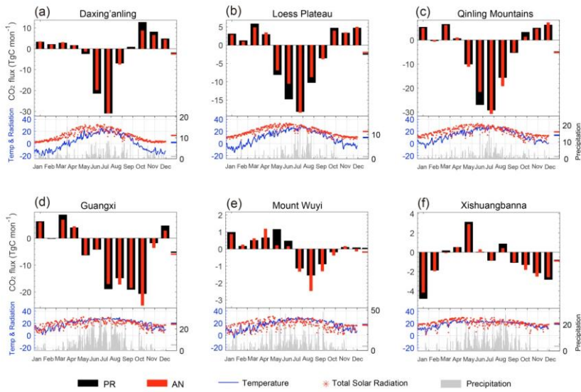
170 Figure 54. Time series of CO 2 biosphere fluxes over six ecological areas of China (blue frames in Fig. 32a; unit: TgC month -1 ), in each month of 2016, obtained from a priori values (PR, black bars) and a posteriori values (AN, red bars). The bars on the right-hand side represent the 12-month average (unit: TgC month -1 ). The subfigures at the bottom denote the daily temperature (blue lines; unit: °C; left-hand y-axis), total solar radiation (red stars; unit: MJ d -1 ; left-hand y-axis), and precipitation (grey bars; unit: mm d -1 ; right-hand y-axis), with the right-hand bars representing the annual average.
