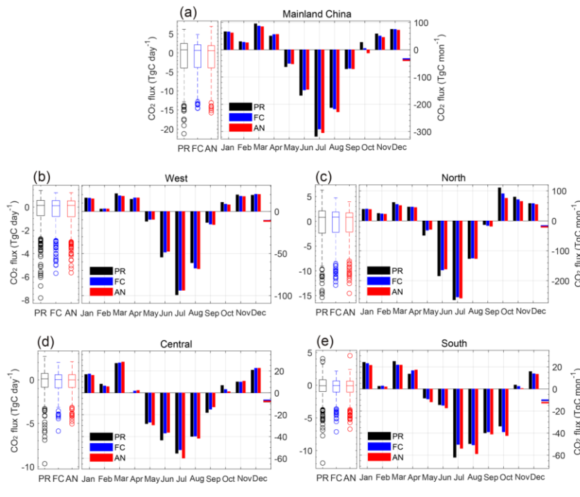
160 Figure 43. Time series of CO 2 biosphere fluxes over (a) mainland China, (b) west China, (c) north 1165 China, (d) central China, and (e) south China, marked by the red frames in Fig. 32a (unit: TgC month -1 ), in each month of 2016, obtained from a priori values (PR, black), a posteriori values (AN, red), and the flux forecast model (FC, blue). The bars on the right-hand side represent the 12-month average (unit: TgC month -1 ). The boxes on the left-hand side denote the daily flux (unit: TgC day -1 ), with the whiskers indicating the minimum and maximum and the horizontal lines across the box indicating the 25 th percentile, the median, and the 75 th percentile, respectively.
