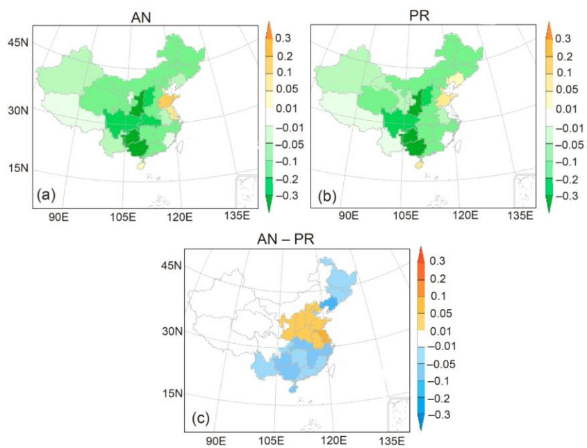
1180 Figure 65. Horizontal distribution of CO 2 biosphere fluxes averaged over each province of mainland China in 2016 (unit: \mu\text{mole m}^{-2} \text{s}^{-1} ): (a) E^a : the a posteriori fluxes; (b) E^p : the a priori fluxes; (c) E^a - E^p : the differences between the a posteriori and a priori CO 2 fluxes. Note that Taiwan, Hong Kong, Macao and Shanghai are not discussed owing to the insufficient grid resolution.
