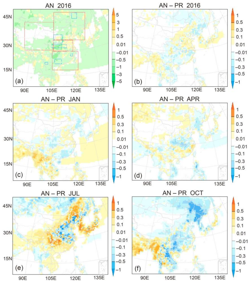
150 Figure 32. Horizontal distribution of CO 2 biosphere fluxes (unit: \mu\text{mole m}^{-2} \text{s}^{-1} ): (a) E^a in 2016, the a posteriori fluxes; (b) E^a - E^p in 2016, the differences between the a posteriori and a priori CO 2 fluxes; 1155 (c) E^a - E^p in January; (d) E^a - E^p in April; (e) E^a - E^p in July; (f) E^a - E^p in October. The red frames mark west China (28°–48°N, 85°–104°E), north China (37°–52°N, 105°–135°E), central China (30°–36°N, 105°–120°E), and south China (18°–29°N, 105°–123°E). The blue frames mark six key ecological areas of China: Daxing'anling (50°–53°N, 121°–127°E); the Loess Plateau (35°–40°N, 105°–112°E); the Qinling Mountains (32°–34°N, 104°–115°E); the rocky desert in Guangxi (22°–25°N, 106°–111°E); Mount Wuyi (26.5°–28.0°N, 117.5°–119.0°E); and Xishuangbanna (21.0°–22.6°N, 100.0°–102.0°E).
