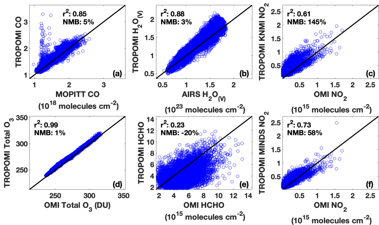
Figure S11: Regression of the indicated species from TROPOMI against retrievals from the satellites listed in Table 1 for May 2018. Both the KNMI (c) and MINDS (f) TROPOMI \text{NO}_2 retrievals are shown. We also indicate the r^2 of a linear least squares fit to the data as well as the normalized mean bias of TROPOMI with respect to the other satellite product.
