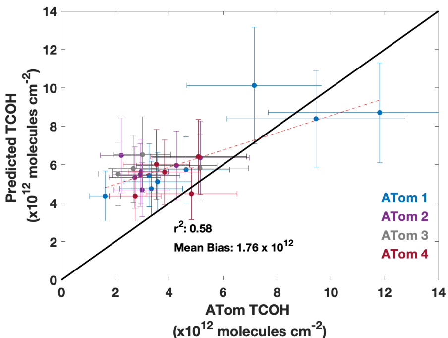
Figure S8: Same as Figure 5 except using \text{NO}_2 calculated with a box model. While there is significant overlap in the columns represented, because of data availability for box modeling, the columns evaluated here are a slightly different subsample of the ATom columns than those shown in Figure 5.
