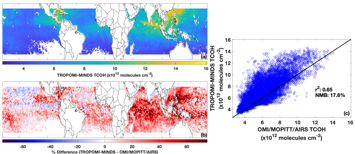
Figure S12: Same as Figure 7 except using the MINDS \text{NO}_2 retrieval for TROPOMI.
