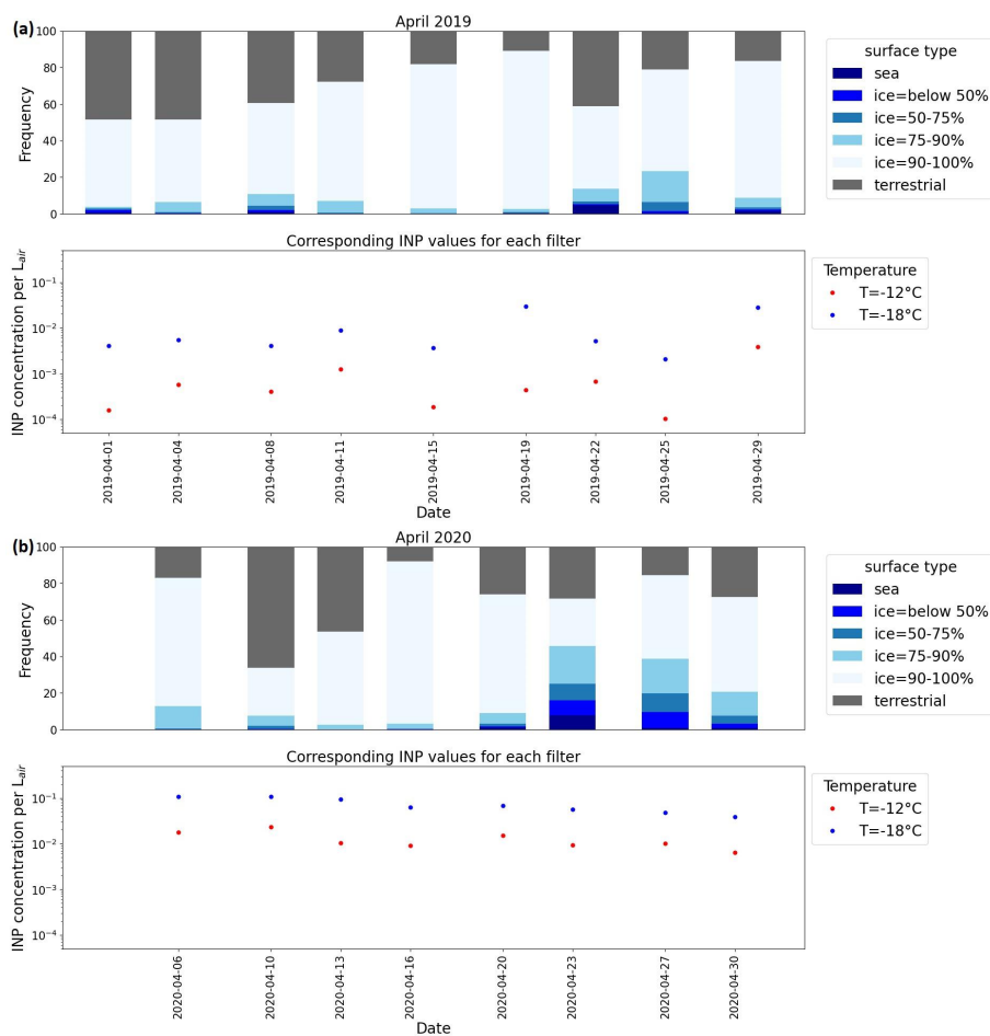
Figure 10. Frequency of the occurrence of different surface types below the trajectory for the sampling period of each filter collected in April 2019 ( a ; upper panel) and April 2020 ( b ; upper panel) are shown as stacked bar plots. Their corresponding INP concentration at -12^{\circ}\text{C} and -18^{\circ}\text{C} are shown in lower panels of ( a ) and ( b ) as reference. Data points are drawn at the end date of the sampling period of each of the 3.5 d filters.
