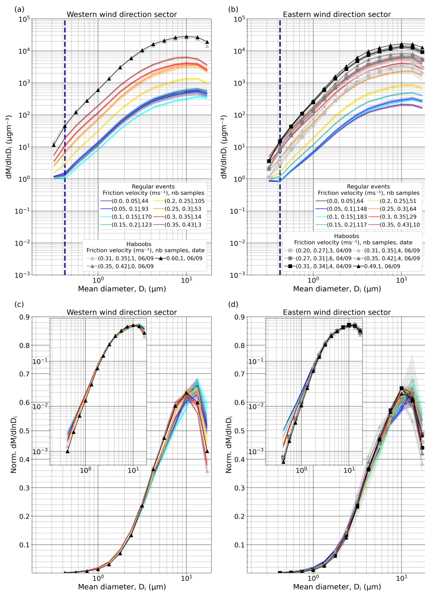
Figure 7. Average size-resolved particle mass concentration, dM/dlnD_i ( \mu\text{g m}^{-3} ), for different u_* intervals, type of event (regular or haboob) and wind directions in the range 150\text{--}330^\circ (a) and 330\text{--}150^\circ (b); The number of available 15-min average PSDs in each u_* interval are indicated in the legend; (c-d) same as (a-b), but normalized ( Norm. dM/dlnD_i ) after removing the anthropogenic mode (normalization from 0.37 to 19.11\ \mu\text{m} ). Insets show the same data, but with logarithmic ordinate axis-scaling. Shaded areas around the lines depict the standard error. The shown PSDs were obtained from FidasL. In (a) and (b) the dark blue dashed line marks the end of the anthropogenic mode ( D_i = 0.42\ \mu\text{m} ). In this case, the original size resolution of FidasL has been reduced by integrating 4 consecutive bins except for the last one that contains three, resulting in 16 bins. First integrated bin is not represented as Fidas is considered efficient from the second one.
