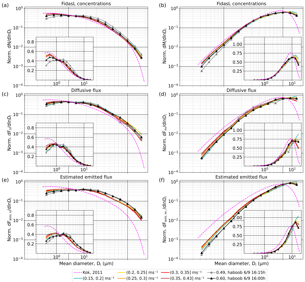
Figure 12. Averaged normalized PSDs considering PSL latex spheres with a refractive index of 1.59 + 0i removing the anthropogenic mode (normalization from 0.37 to 19.11 \mu\text{m} ) for well-developed erosion conditions during regular events and for two PSDs during haboob events for FidasL (a-b), for diffusive flux (c-d) and for estimated emitted flux using the v_{dep} from the tuned parameterization (e-f). (a,c,e) show \text{Norm. } dN/d\ln D_i and (b,d,f) \text{Norm. } dM/d\ln D_i . The insets show the same data, but the scale of the ordinate is linear. Pink dashed lines represent the invariant Kok (2011a) size distribution. The original size resolution of FidasL has been reduced by integrating 4 consecutive bins except for the last one that contains three, resulting in 16 bins. First integrated bin is not represented as Fidas is considered efficient from the second one.
