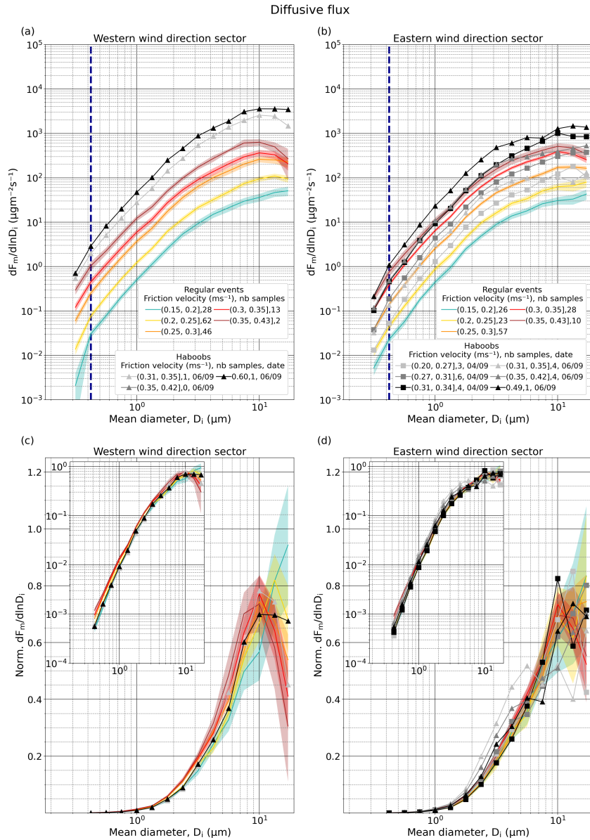
Figure 9. Average size-resolved mass diffusive flux, dF_m/dlnD_i ( \mu\text{g m}^{-2} \text{s}^{-1} ), for different u_* intervals, type of event (regular or haboob) and wind directions in the range 150\text{--}330^\circ (a) and 330\text{--}150^\circ (b); The number of available 15-min average PSDs in each u_* class are indicated in the legend. Only the samples where diffusive flux is positive in all the diameter bins above the anthropogenic mode (as discussed in Sect. 3.3.1) have been selected; (c-d) same as (a-b), but normalized ( Norm. dF_m/dlnD_i ) after removing the anthropogenic mode (normalization from 0.37 to 19.11 \mu\text{m} ). Insets show the same data, but with logarithmic ordinate axis-scaling. Shaded areas around the lines of the regular events PSDs illustrate the combination of random uncertainty and standard error. In (a) and (b) the dark blue dashed line marks the end of the anthropogenic mode ( D_i = 0.42 \mu\text{m} ). In this case, the original size resolution of FidasL has been reduced by integrating 4 consecutive bins except for the last one that contains three, resulting in 16 bins. First integrated bin is not represented as Fidas is considered efficient from the second one. Results are shown only for well-developed erosion conditions ( u_* > 0.15 \text{ m s}^{-1} ).
