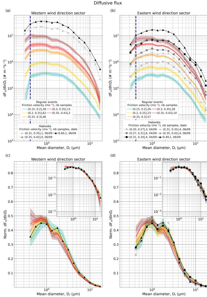
Figure 8. Average size-resolved number diffusive flux, dF_n/d\ln D_i ( \# \text{ m}^{-2} \text{ s}^{-1} ), for different u_* intervals, type of event (regular or haboob) and wind directions in the range 150\text{--}330^\circ (a) and 330\text{--}150^\circ (b); The number of available 15-min average PSDs in each u_* interval are indicated in the legend. Only the samples where diffusive flux is positive in all the diameter bins above the anthropogenic mode (as discussed in Sect. 3.3.1) have been selected; (c-d) same as (a-b), but normalized (Norm. dF_n/d\ln D_i ) after removing the anthropogenic mode (normalization from 0.37 to 19.11 \mu\text{m} ). Insets show the same data, but with logarithmic ordinate axis-scaling. Shaded areas around the lines of the regular events PSDs depict the combination of random uncertainty and standard error. In (a) and (b) the dark blue dashed line marks the end of the anthropogenic mode ( D_i = 0.42 \mu\text{m} ). In this case, the original size resolution of FidasL has been reduced by integrating 4 consecutive bins except for the last one that contains three, resulting in 16 bins. First integrated bin is not represented as Fidas is considered efficient from the second one. Results are shown only for well-developed erosion conditions ( u_* > 0.15 \text{ m s}^{-1} ).
