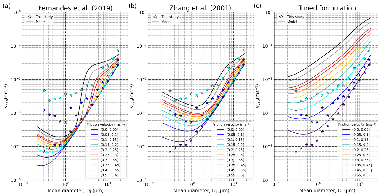
Figure 10. Median size-resolved dry deposition velocities v_{dep}(\text{m s}^{-1}) obtained applying (a) F19, (b) Z01 and (c) tuned parameterization and using field measurements, for different u_* intervals (solid lines). The stars correspond to the median of the observationally-based v_{dep} for the u_* intervals (0 - 0.05] \text{ m s}^{-1} (purple), (0.05 - 0.10] \text{ m s}^{-1} (blue) and (0.10 - 0.15] \text{ m s}^{-1} (cyan).
