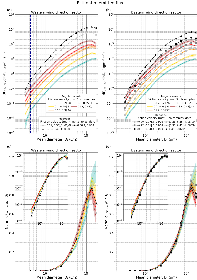
Figure 11. Average size-resolved mass estimated emitted flux, dF_{emi.m.}/dlnD_i ( \mu\text{g m}^{-2} \text{s}^{-1} ), for different u_* intervals, type of event (regular or haboob) and wind directions in the range 150\text{--}330^\circ (a) and 330\text{--}150^\circ (b); The number of available 15-min average PSDs in each u_* class are indicated in the legend. Only the samples where diffusive flux is positive in all the diameter bins above the anthropogenic mode (as discussed in Sect. 3.3.1) have been selected; (c-d) same as (a-b), but normalized ( Norm. dF_{emi.m.}/dlnD_i ) after removing the anthropogenic mode (normalization from 0.37 to 19.11 \mu\text{m} ). Insets show the same data, but with logarithmic ordinate axis-scaling. Shaded areas around the lines of the regular events PSDs illustrate the combination of random uncertainty and standard error. In (a) and (b) the dark blue dashed line marks the end of the anthropogenic mode ( D_i = 0.42 \mu\text{m} ). In this case, the original size resolution of FidasL has been reduced by integrating 4 consecutive bins except for the last one that contains three, resulting in 16 bins. First integrated bin is not represented as Fidas is considered efficient from the second one. Results are shown only for well-developed erosion conditions ( u_* > 0.15 \text{m s}^{-1} ).
