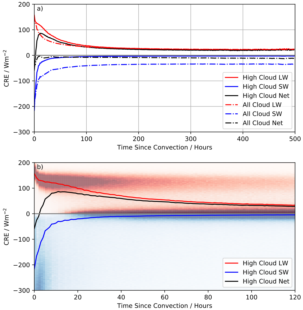
Figure 10. Cloud Radiative Effect (CRE) as a function of TSC. a) All cloud and high cloud LW, SW and Net CRE up to 500 hours from convection. b) High cloud only LW, SW and Net CRE up to 120 hours from convection with normalised joint histogram the showing the probability of finding a particular CRE value (LW in red, SW in blue) for a given TSC value.
