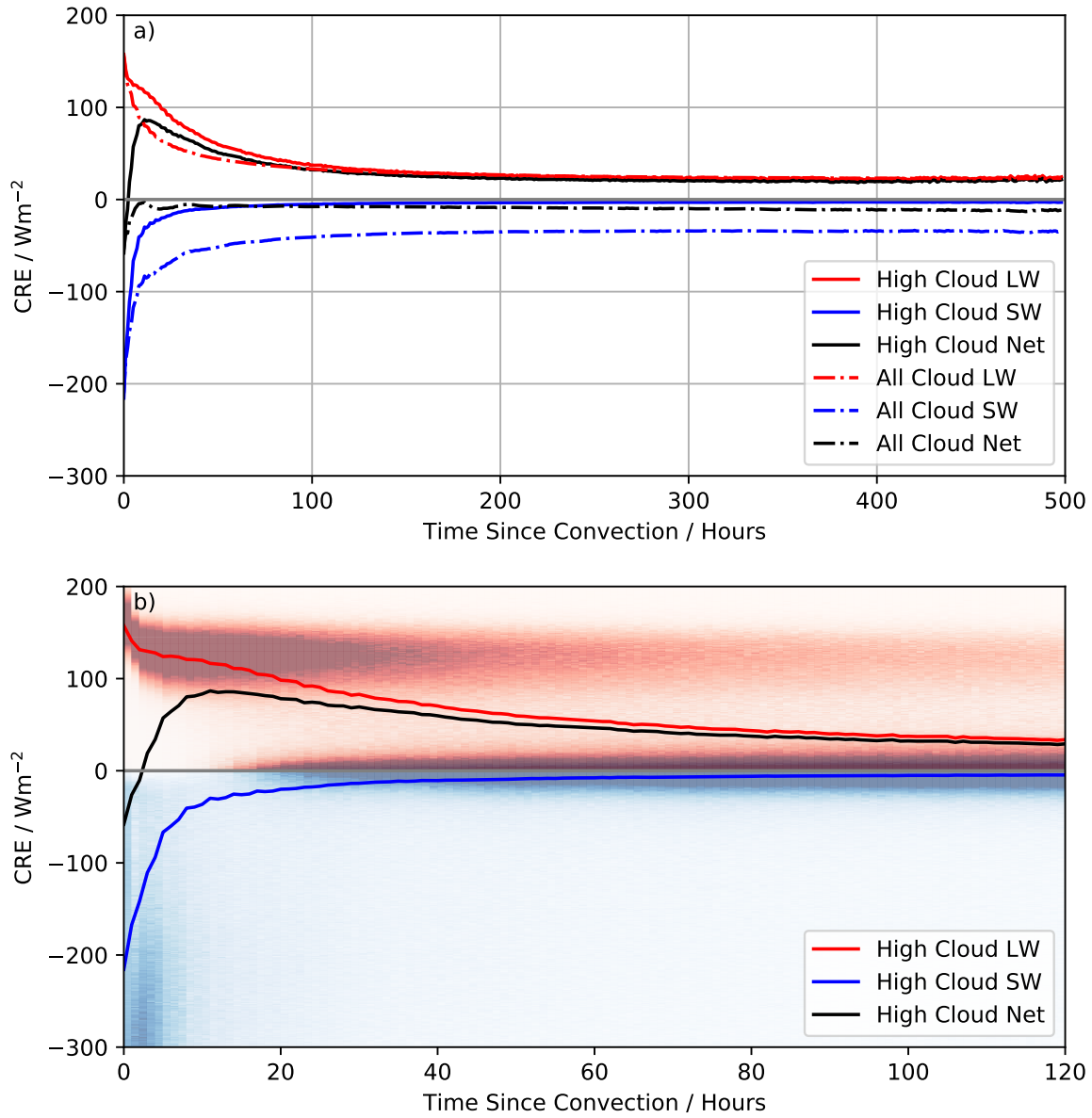
Figure 10. Cloud Radiative Effect (CRE) as a function of TSC. a) All cloud and high cloud LW, SW and Net CRE up to 500 hours from convection. b) High cloud only -LW, SW and Net CRE up to 120 hours from convection with normalised joint histogram the showing the probability of finding a particular CRE value (LW in red, SW in blue) for a given TSC value.
