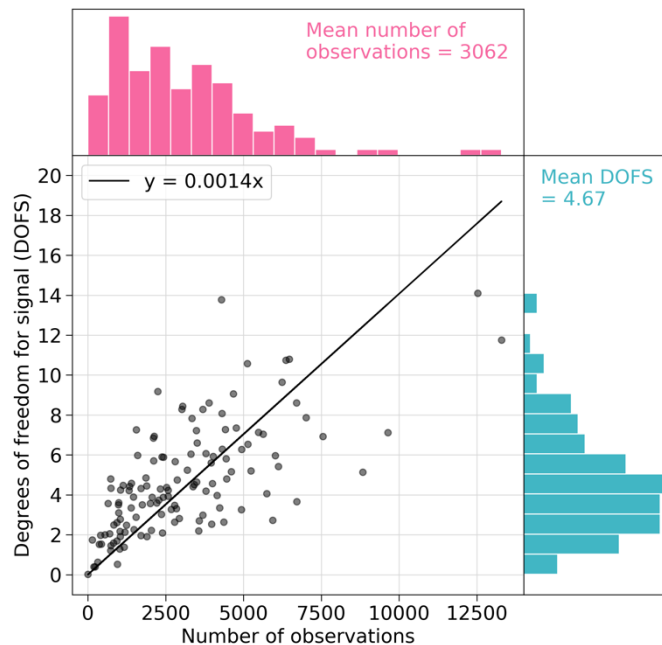
230 Figure 4: Weekly information content of TROPOMI observations over the Permian Basin. The figure shows the dependence of the weekly degrees of freedom for signal (DOFS) for the inversion on the weekly number of TROPOMI observations in the Permian region of interest (Figure 1), for 127 weeks of inversions. The DOFS represent the number of independent pieces of information on the emission distribution that can be quantified by the inversion independently from the prior estimate. The top histogram shows the distribution of weekly observation counts in the Permian. The right histogram shows the distribution of weekly DOFS in the Permian. Also shown is the 235 reduced-major-axis regression line, indicating 1.4 DOFS per 1000 TROPOMI observations.
