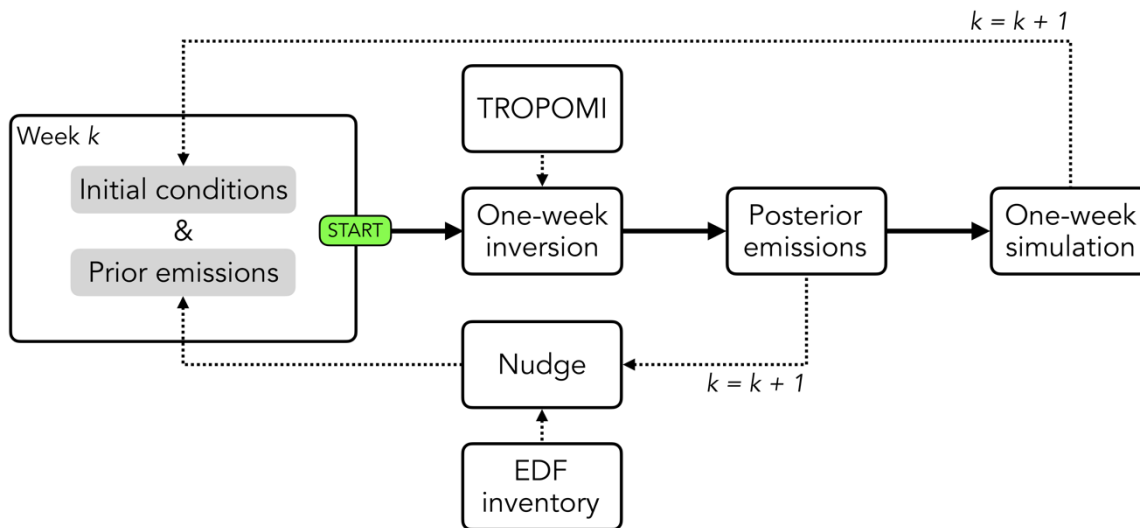
175 Figure 2: Flowchart of our Kalman filter inversion methodology for estimating weekly emissions. Starting from a set of initial conditions and prior emission estimates for the inversion domain (Figure 1), a one-week inversion produces posterior emission estimates for week k . The posterior emission estimates are then nudged towards the original EDF inventory emissions before substitution to serve as prior estimates for week k+1 , and are used in a one-week simulation for week k to generate initial conditions for week k+1 .
