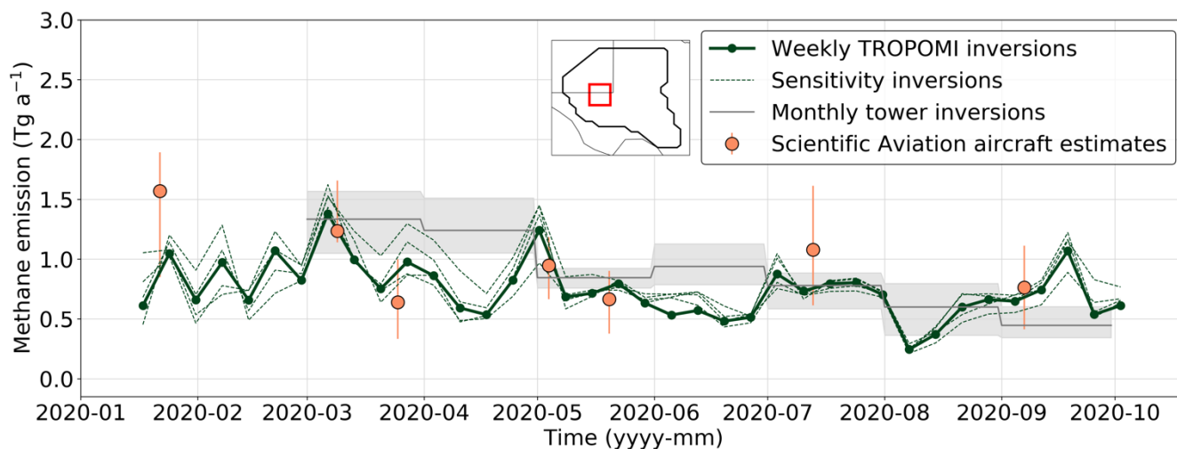
270 Figure 6: Weekly methane emissions from the Lyon et al. (2021) PermianMAP study region (red box in inset: 103.2^{\circ} – 104.2^{\circ} W, 31.4^{\circ} – 32.4^{\circ} N). Results from our weekly TROPOMI inversions are compared to monthly tower inversions and aircraft model-based scaling-factor estimates reported by Barkley et al. (2022). The grey shaded area and orange bars represent sensitivity ranges.
