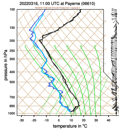
d) Vertical profiles from ACI-dusty simulation
