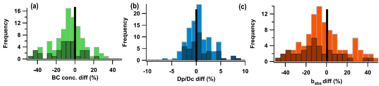
Figure. 7 Histogram of the number frequency of the relative differences between 240 m and the ground for a) BC, (b) D_p/D_c and (c) b_{abs} . The shaded black area denotes the number frequency at night and morning (6:00,7:00, 8:00, 22:00, 23:00), the black line denotes no difference between 240m and the ground.
