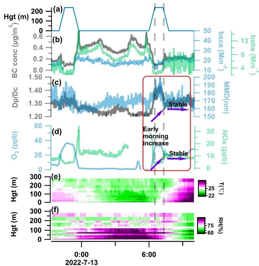
655 Figure. 6 A typical case of vertical mixing from the residual layer leading to an increase in O_3 and D_p/D_c in the early morning. (a) The height of moveable container. (b)-(d) Time series (1-min resolution) of BC mass concentration, b_{abs} , b_{sca} , D_p/D_c , MMD, O_3 and NO_x . (e) 2D (height and time) plot of temperature, the colours denote the quantity of the temperature. (f) The same as e, but for relative humidity.
