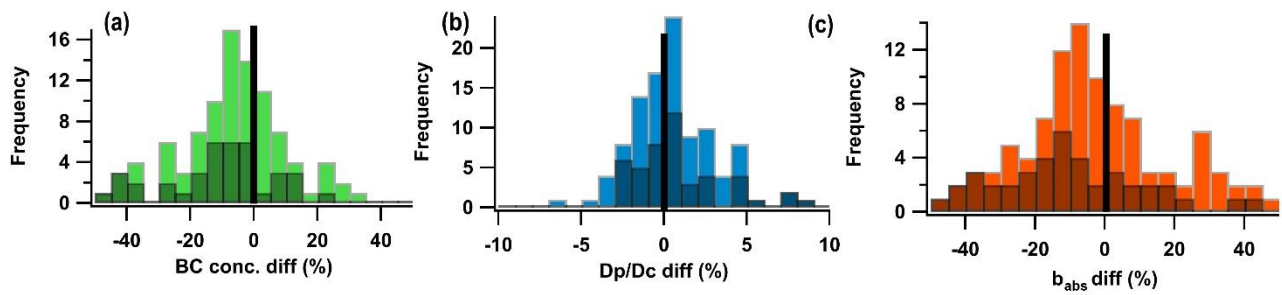
Figure. 7 Histogram of the number frequency of the relative differences between 240 m and the ground for a) BC, (b) D_p/D_c and (c) b_{abs} . The shaded black area denotes the number frequency at night and morning (6:00,7:00, 8:00, 22:00, 23:00), the black line denotes no difference between 240m and the ground.
