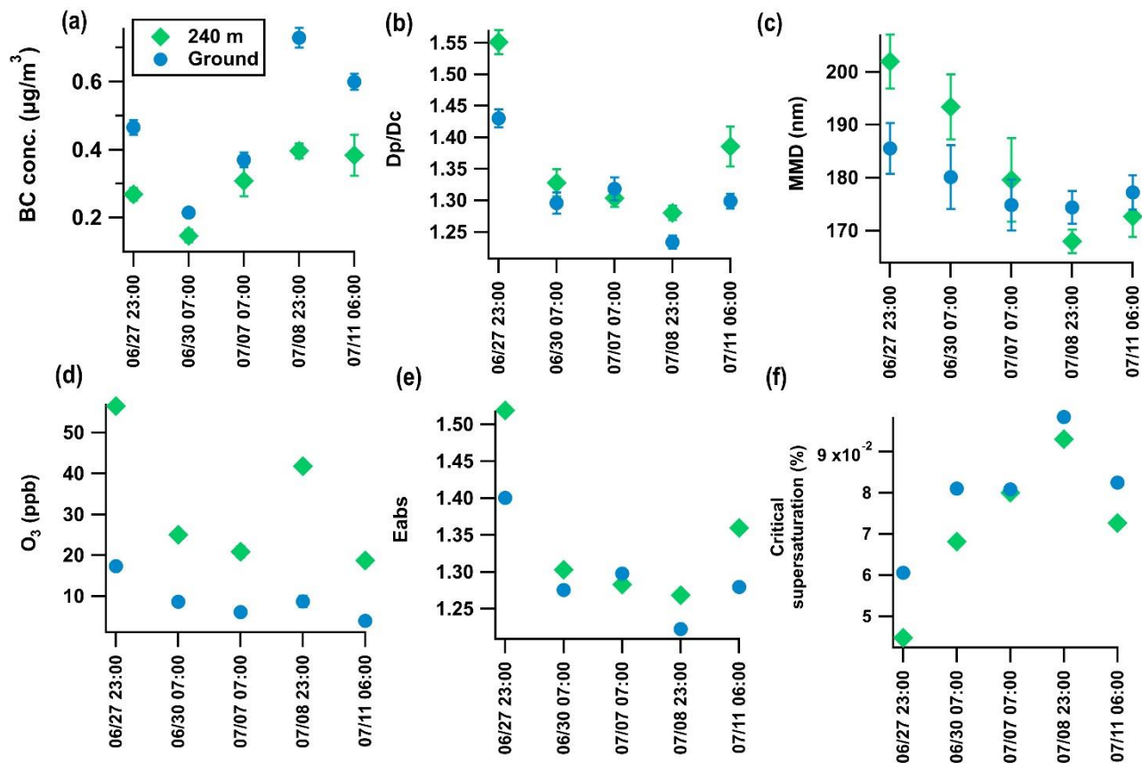
Figure. 5 Comparison between the surface and 240 m height in the sharp decrease type of major pollutant
